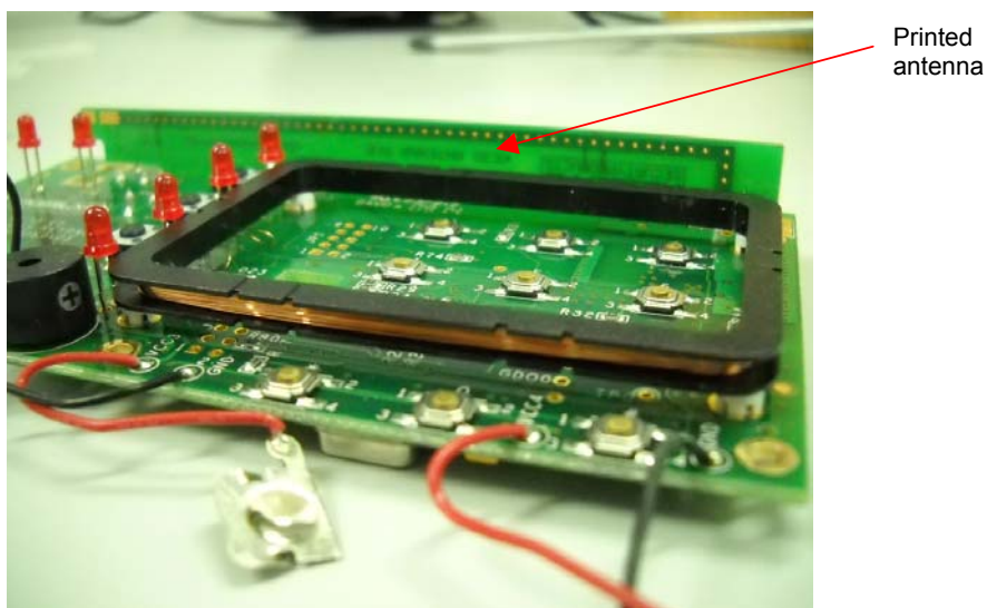
Photograph 7.4.1 Antenna assembly
