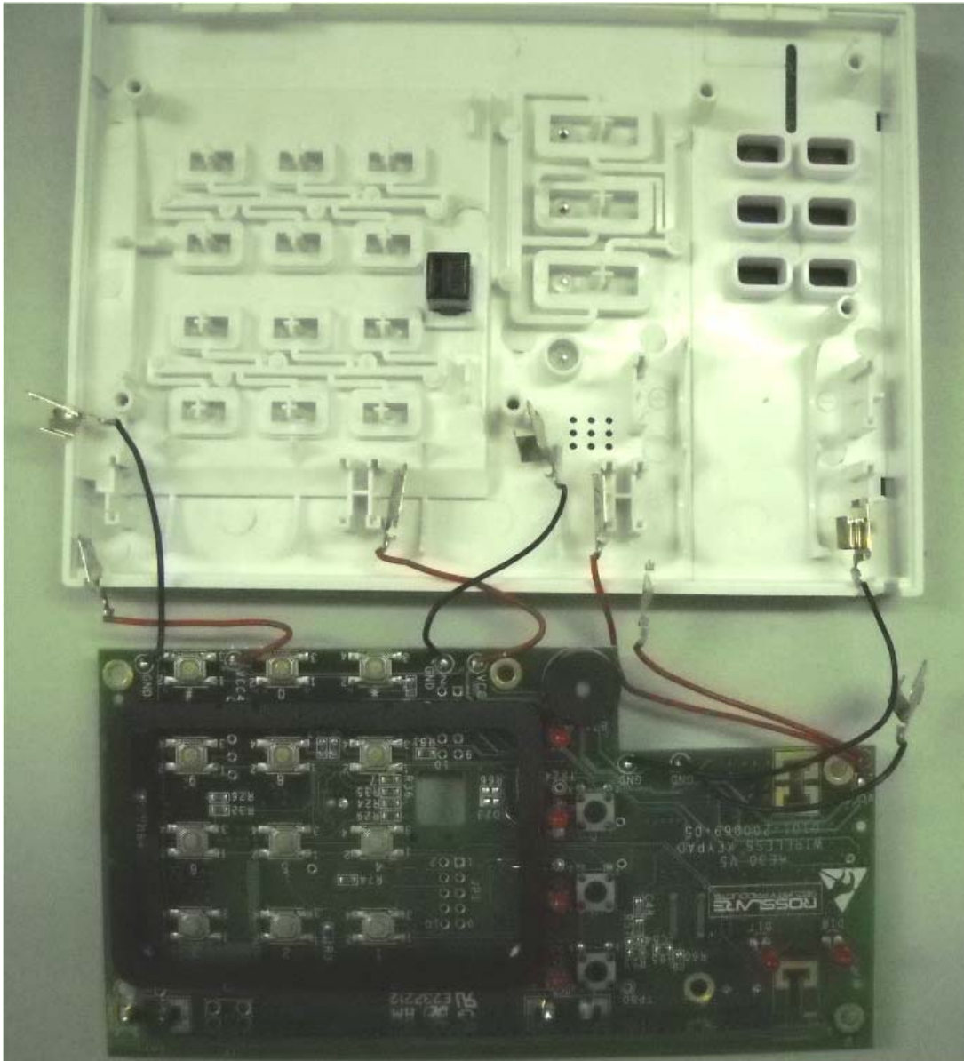
Photograph No.2 KE-30G keypad internal view
