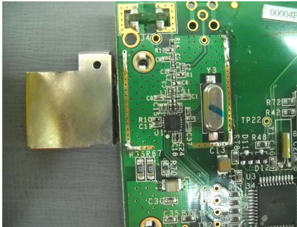
Photograph No.8 PCB without shielding
