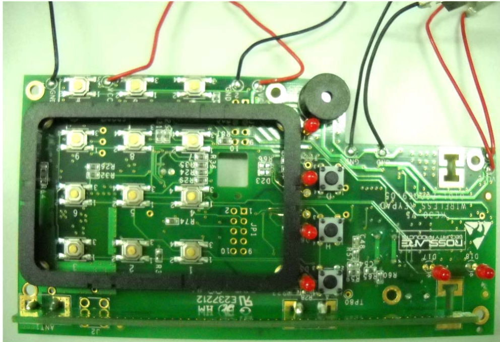
Photograph No.4 KE-30G keypad PCB second side view
