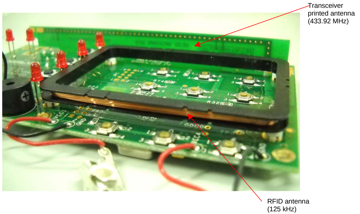
Photograph No.6 KE-30G keypad RFID antenna
