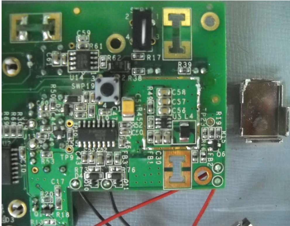
Photograph No.7 PCB without shielding
