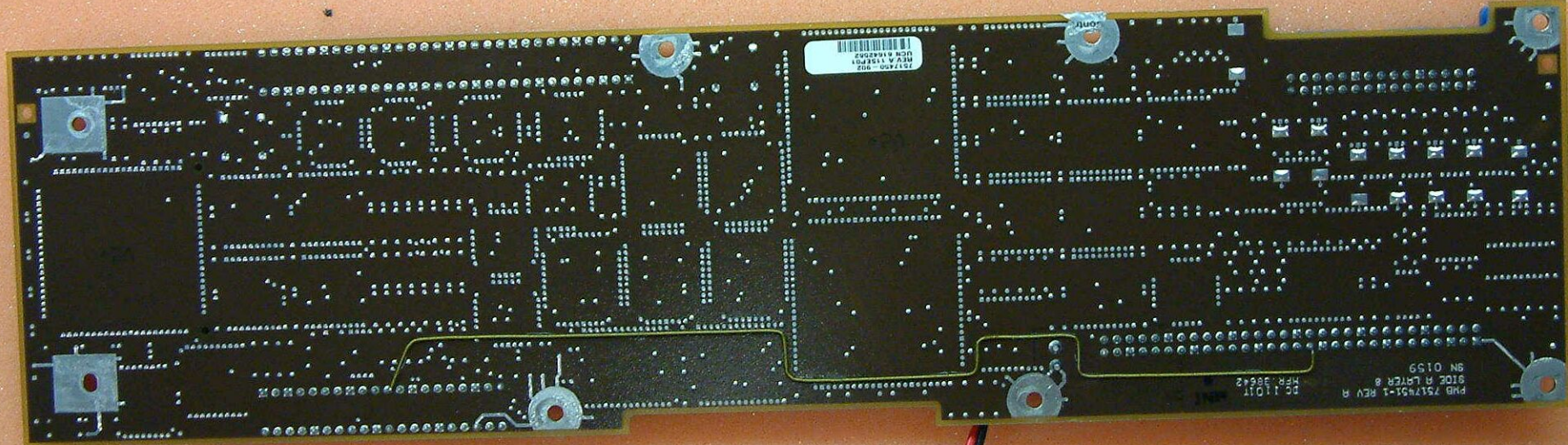
7517450-902, DADC/IAC processor, rear view
