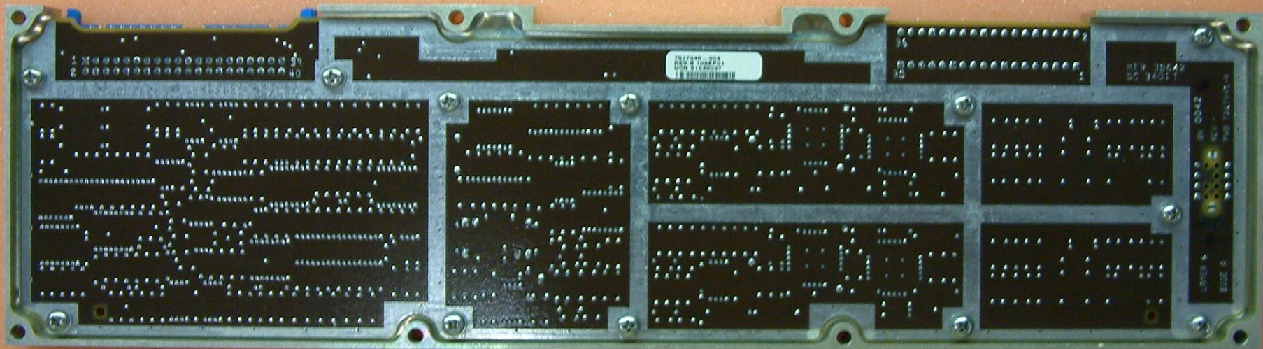
7517440-904, Transponder receiver, rear view
