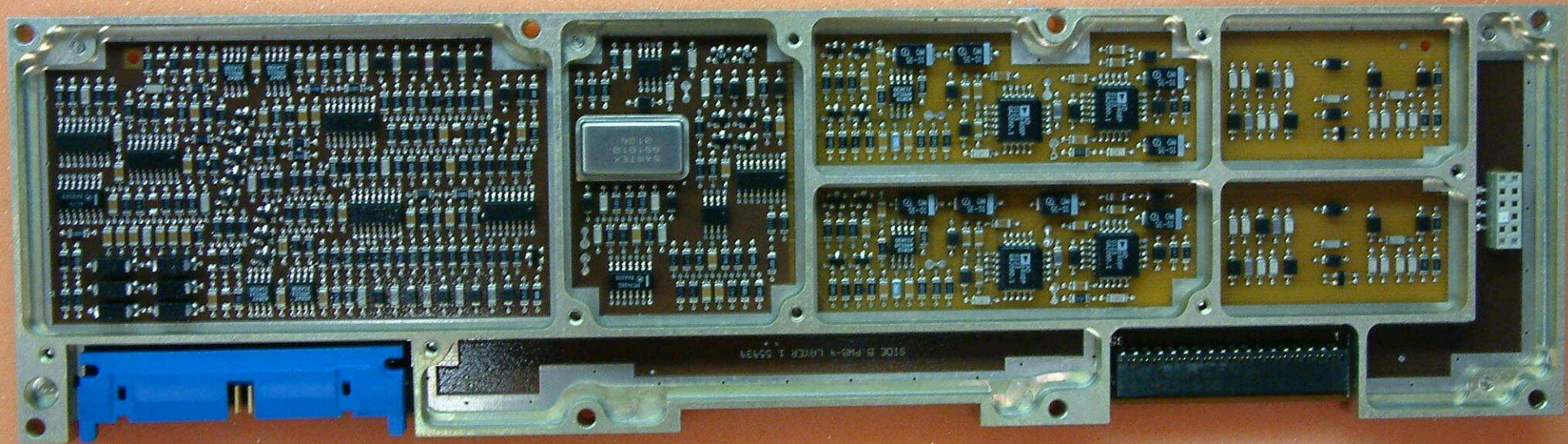
7517440-904, transponder receiver, front view
