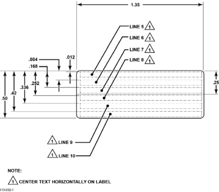
FIGURE 6. OUTLINE
