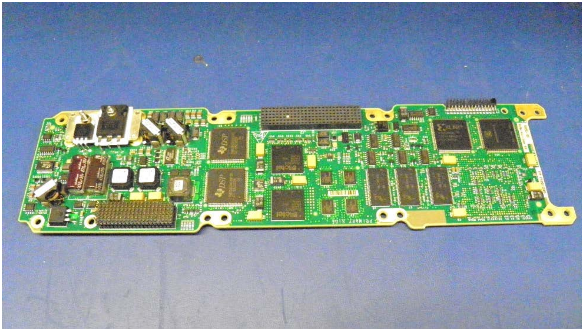
CPU / PS PBA – Top Side
