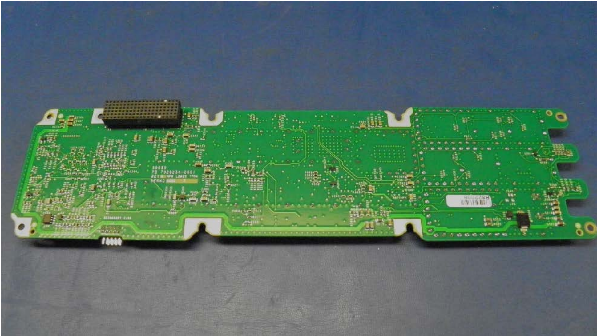
VHF RX PBA – Bottom Side
