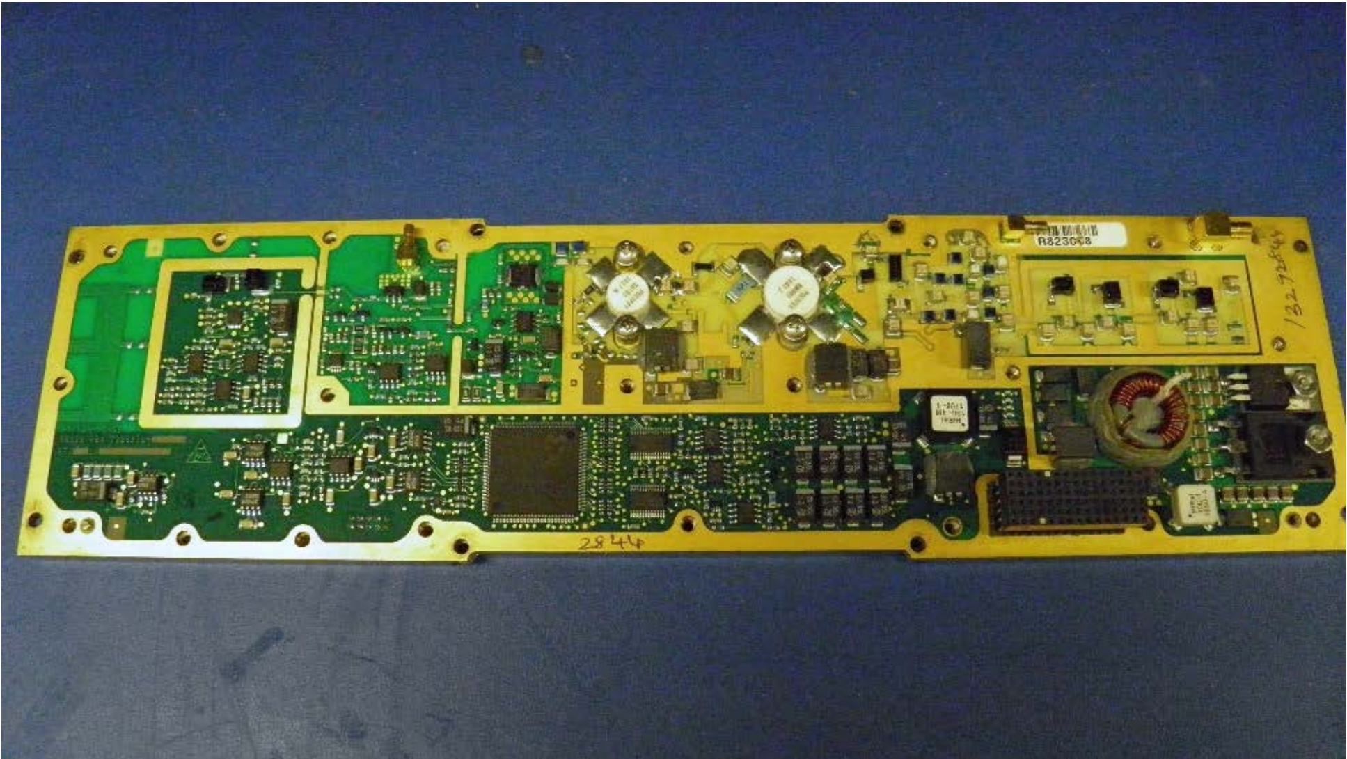
VHF TX PBA – Top Side
