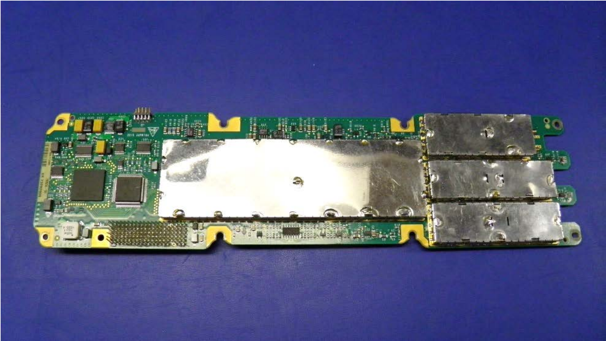
VHF RX PBA – Top Side
