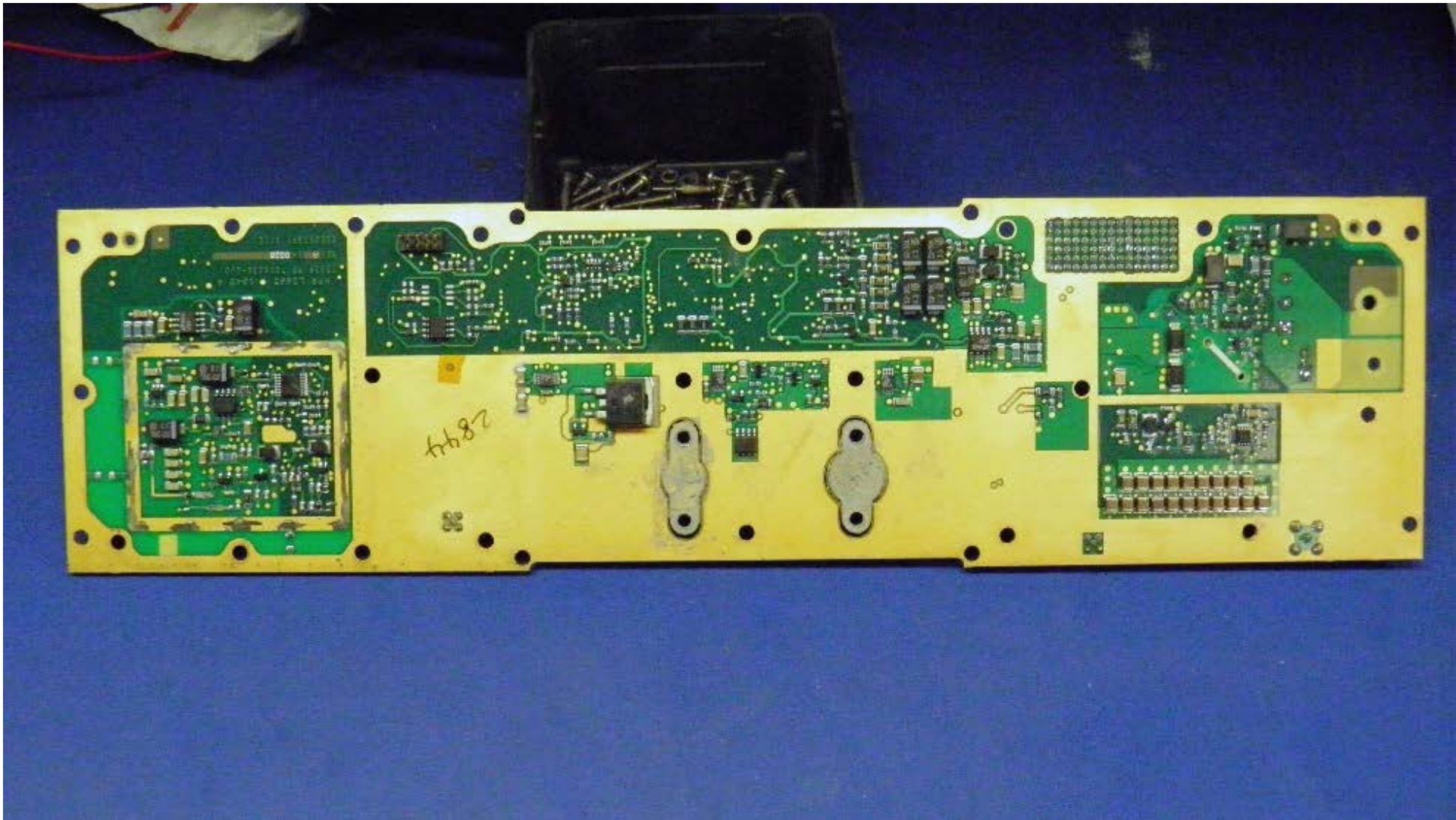
VHF TX PBA – Bottom Side
