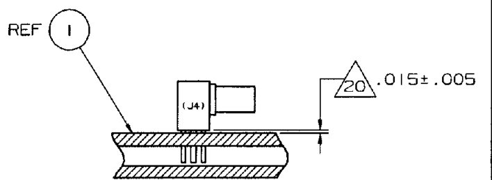
SECTION F-F
