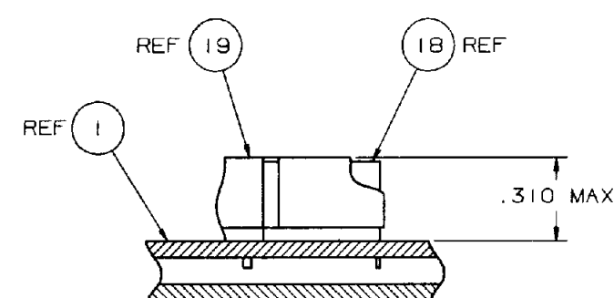
SECTION G-G
