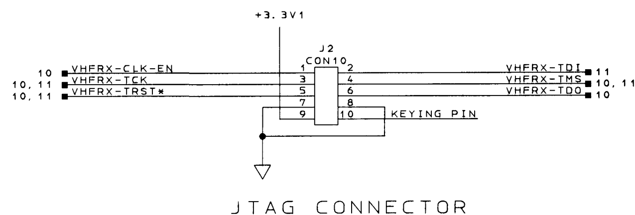
JTAG CONNECTOR
