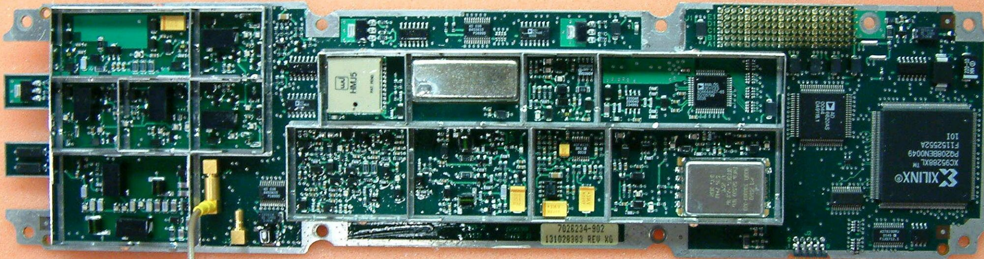
7026234-902, VHF receiver, front view
