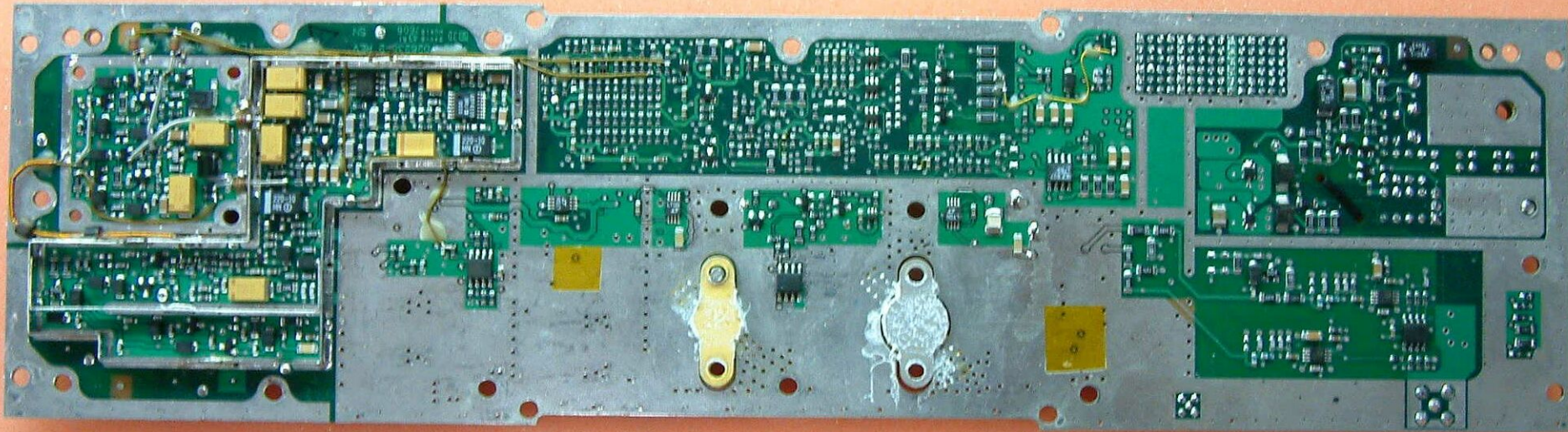
7026236-902, Transmitter, rear view
