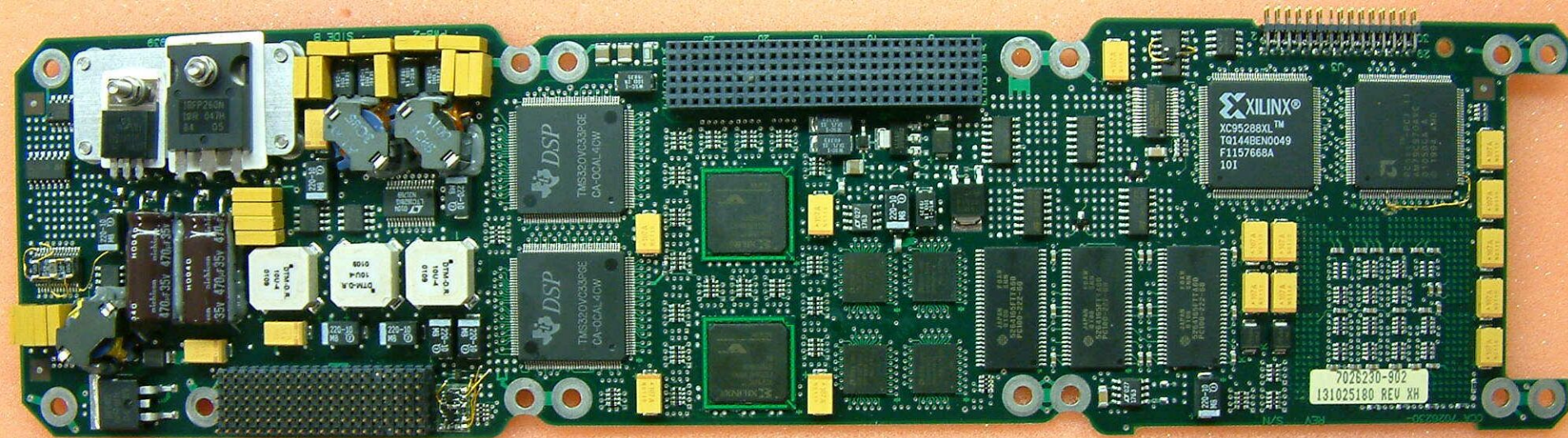
7026230-902, Power supply/CPU, front view
