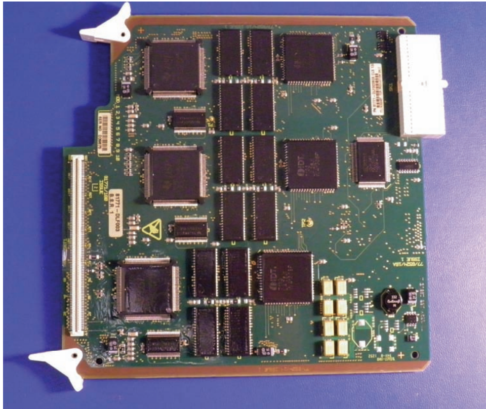
Triple Transcoder Module (TTCM) – Side 1
