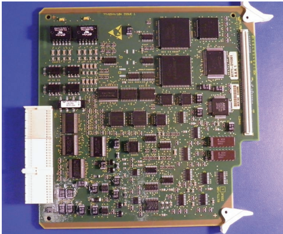
Voice Interface Module (VIM) – Side 1
