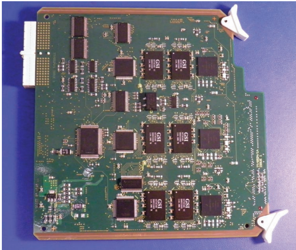
Triple Transcoder Module (TTCM) – Side 2
