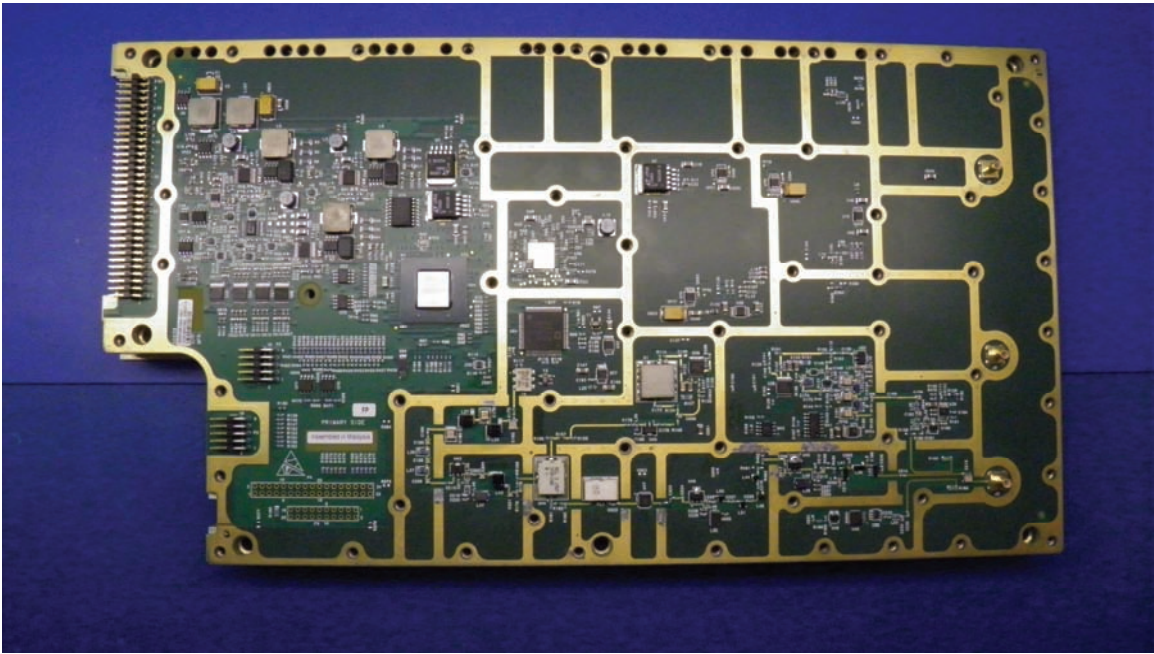
Radio Frequency Module - Circuit Card Assembly - Side 1
