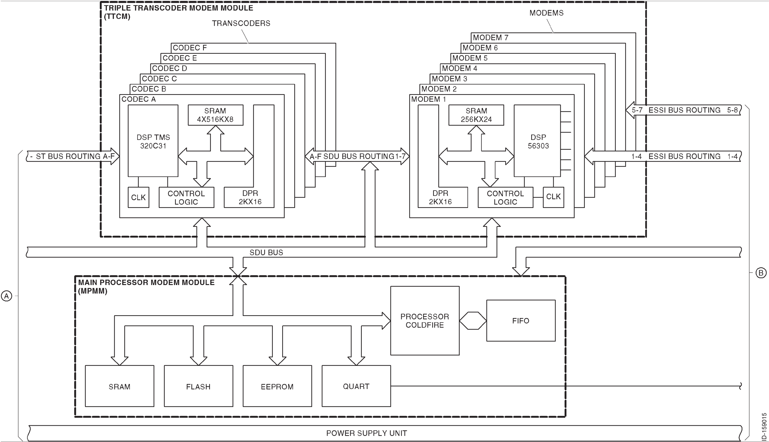
Figure 6. (Sheet 2 of 3) SDU Functional Diagram (GRAPHIC 23-20-26-99B-809-A01)
