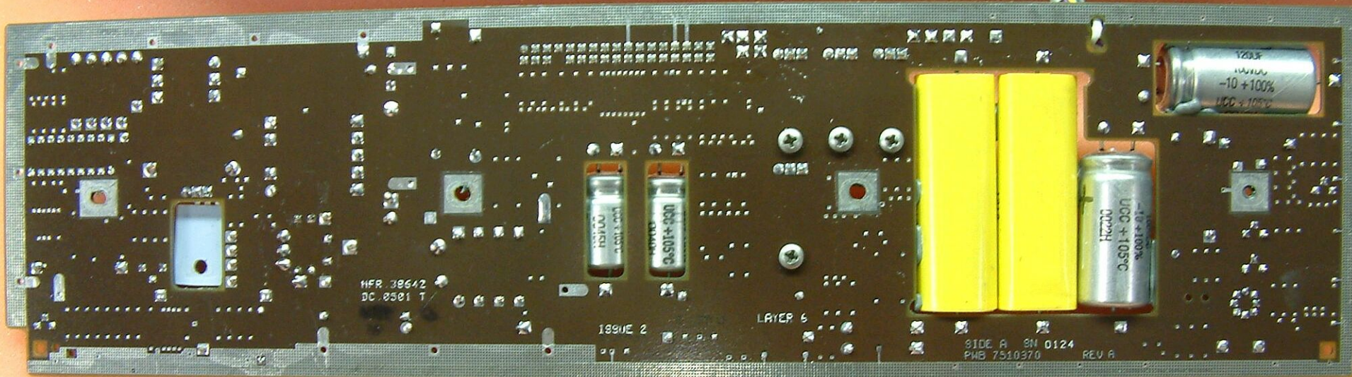
7510220-902, DME modulator/ power supply, rear view
