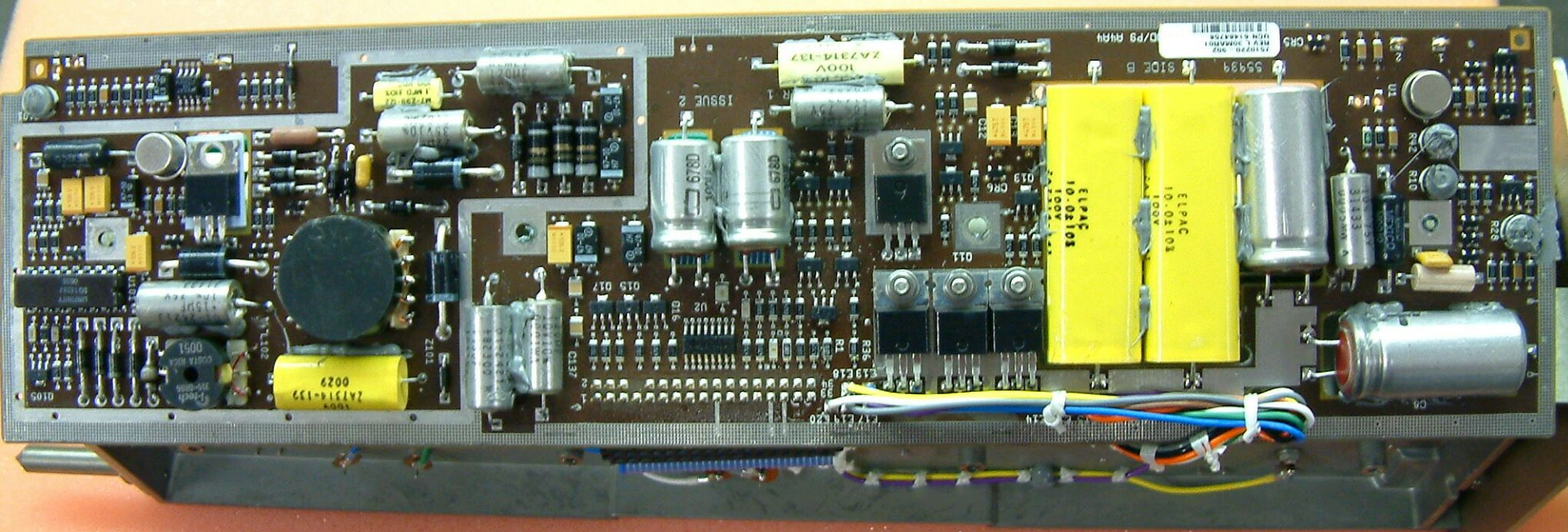
7510220-902, DME modulator/ power supply, front view
