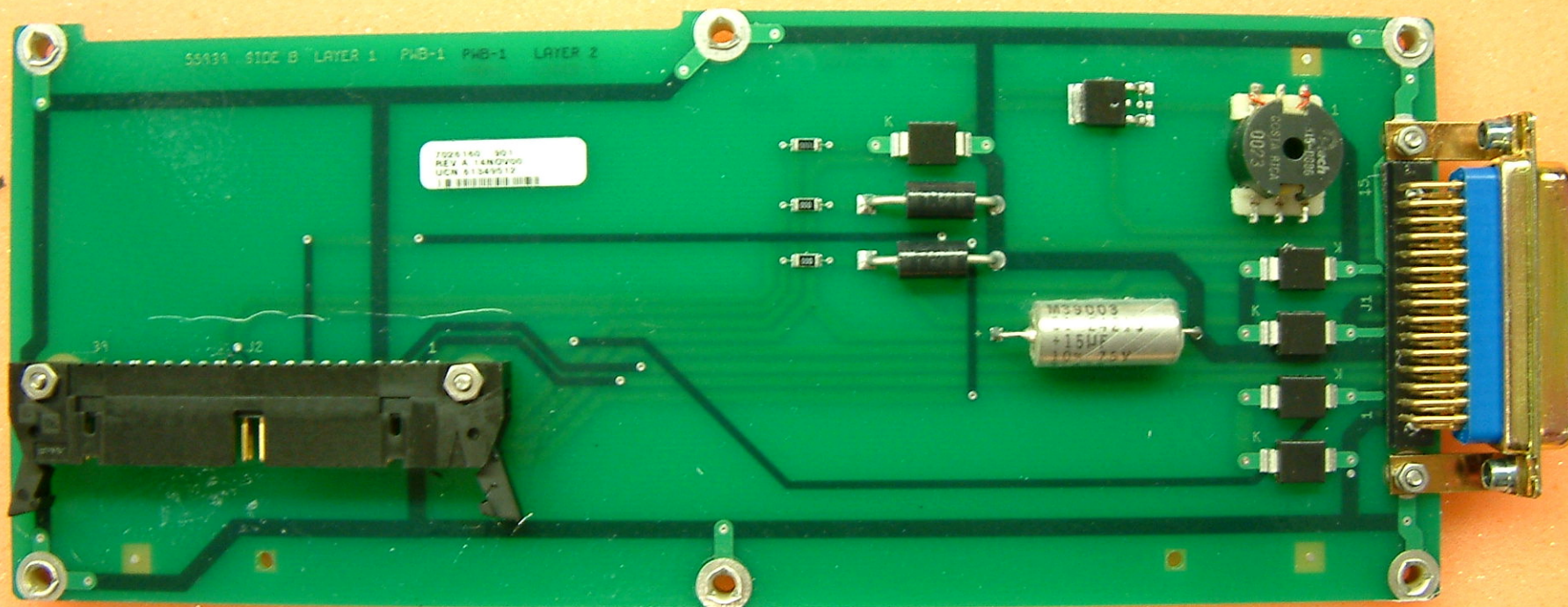
7026160-901, DME Interface, Front view
