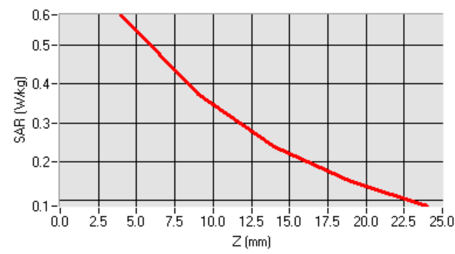
SAR, Z Axis Scan (X = -2, Y = -6)
