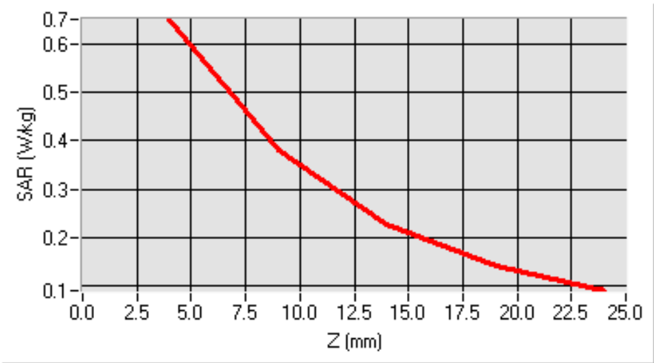
SAR, Z Axis Scan (X = -9, Y = 1)
