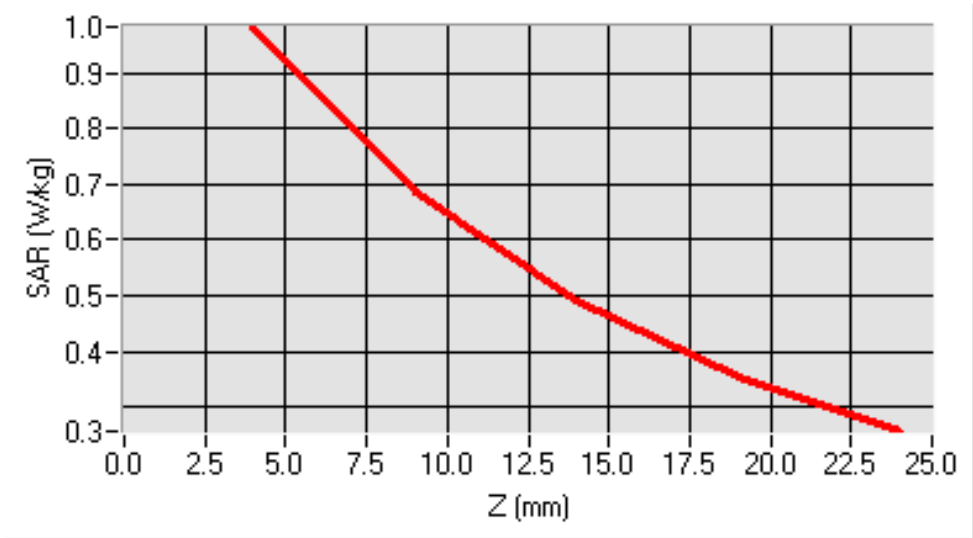
SAR, Z Axis Scan (X = -29, Y = -13)
