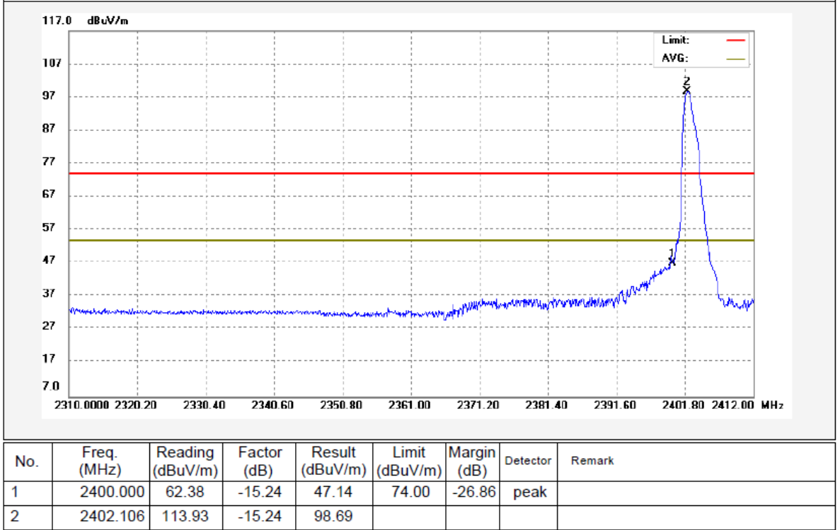
8DPSK Transmitting Band edge-left side Vertical
