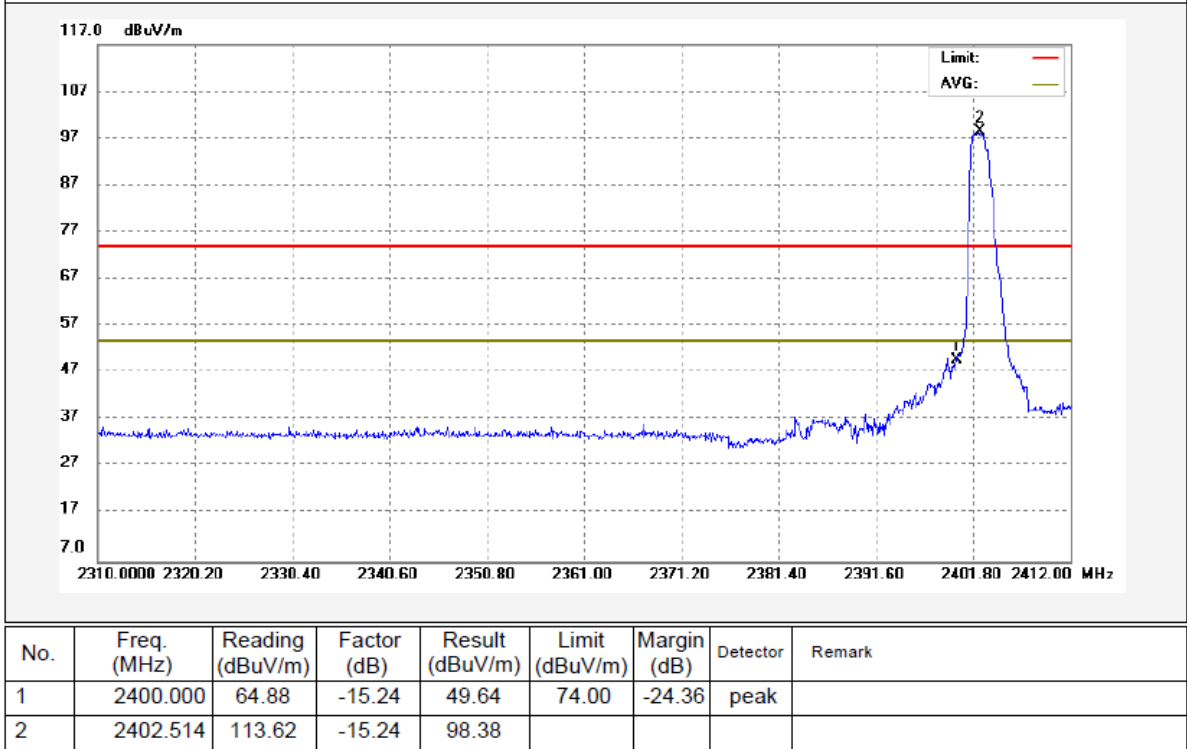
8DPSK Transmitting Band edge-left side Horizontal
