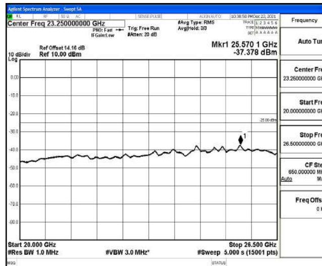
Band7-20MHz-16QAM-21350-1RB#0-Range6:20000~26500MHz
