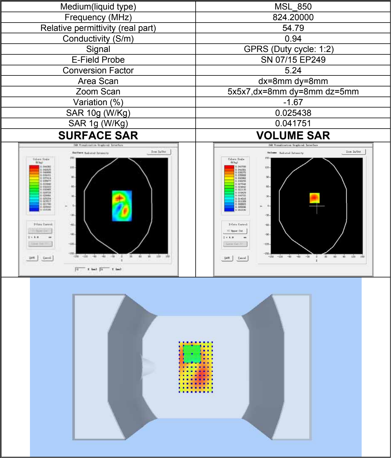
Plot 9: GPRS850MHz, Low channel(Body-worn, Bottom edge) Product Description: MOBILE PHONE Test Date: 2018-04-12
