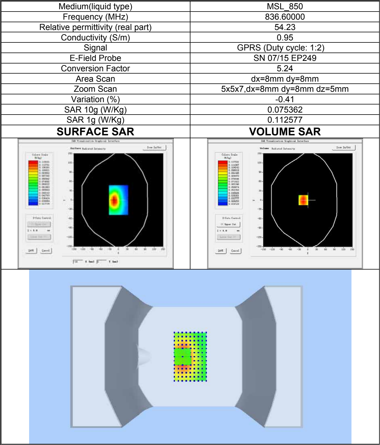
Plot 9: GPRS850MHz, Mid channel(Body-worn, Bottom edge) Product Description: MOBILE PHONE Test Date: 2018-03-05
