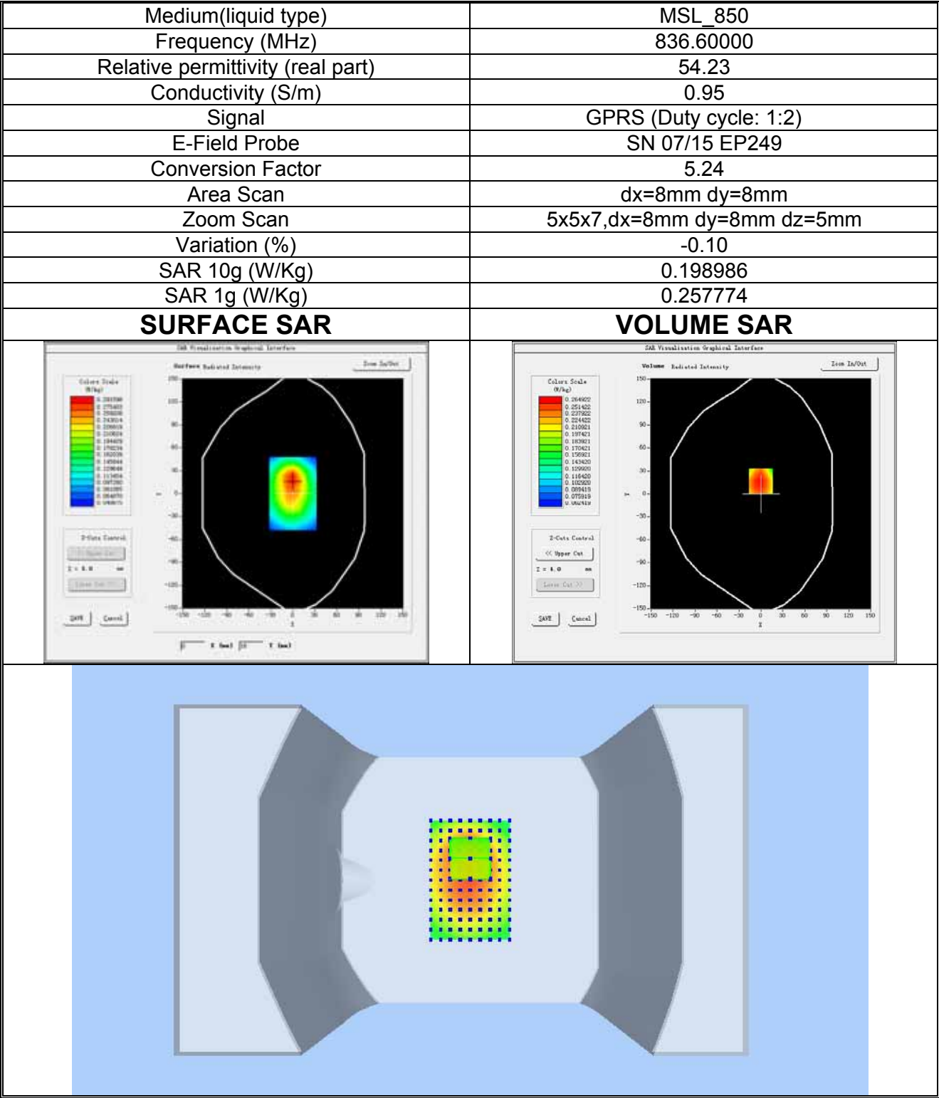
Plot 8: GPRS850MHz, Mid channel(Body-worn, Left edge) Product Description: MOBILE PHONE Test Date: 2018-03-05
