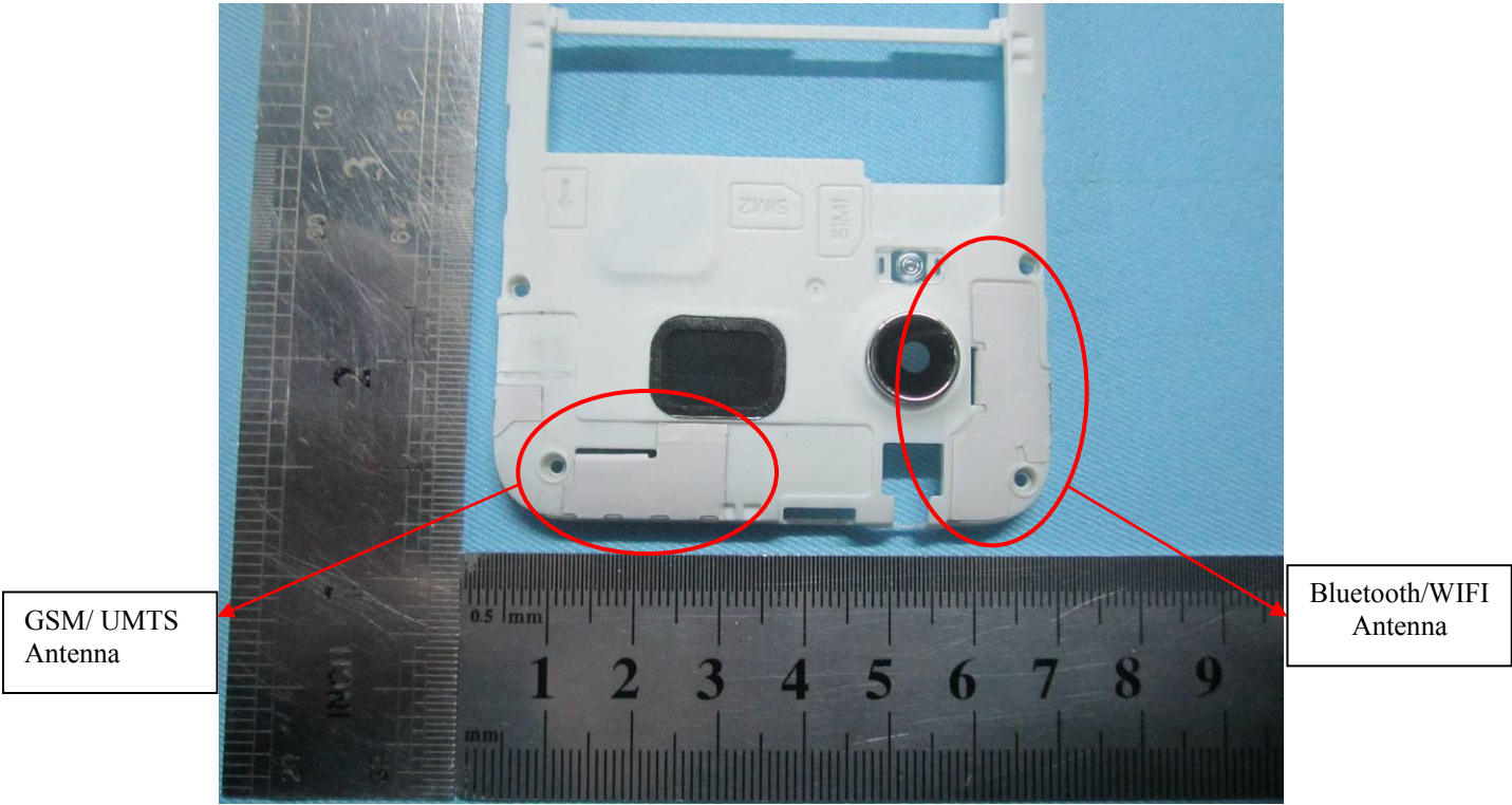
Antenna View
