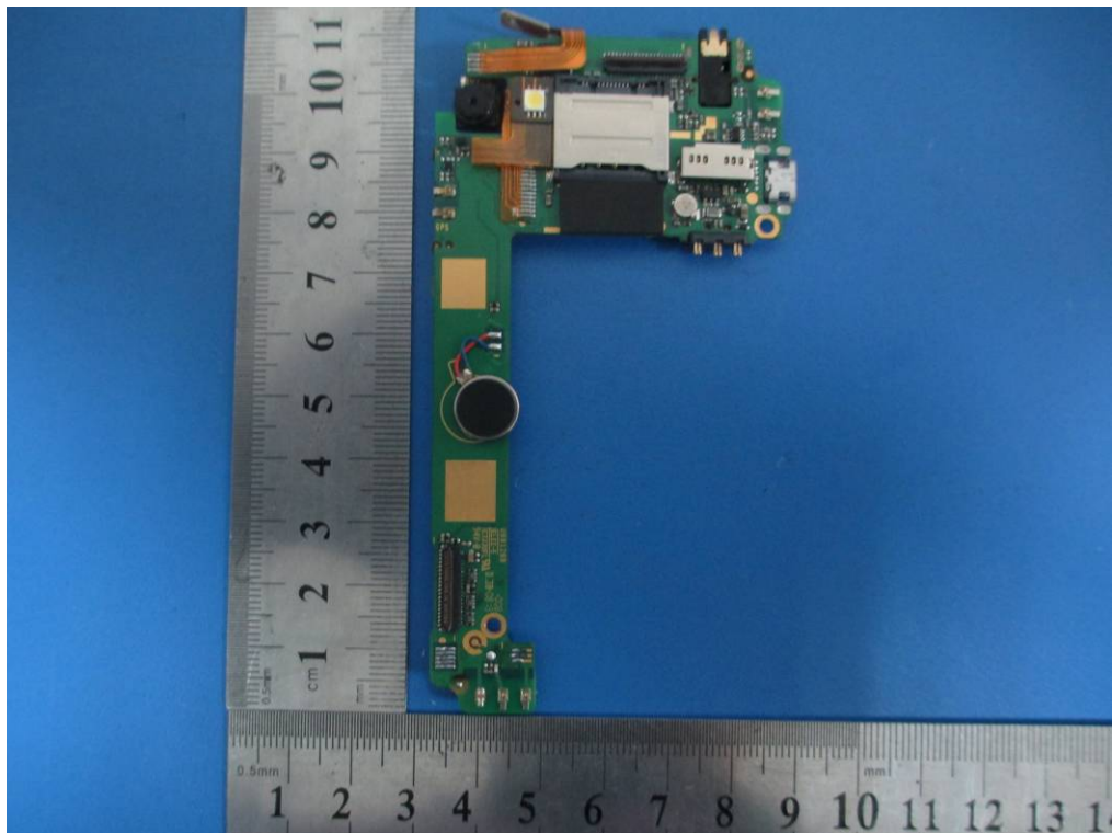
Top - PCB 1#
