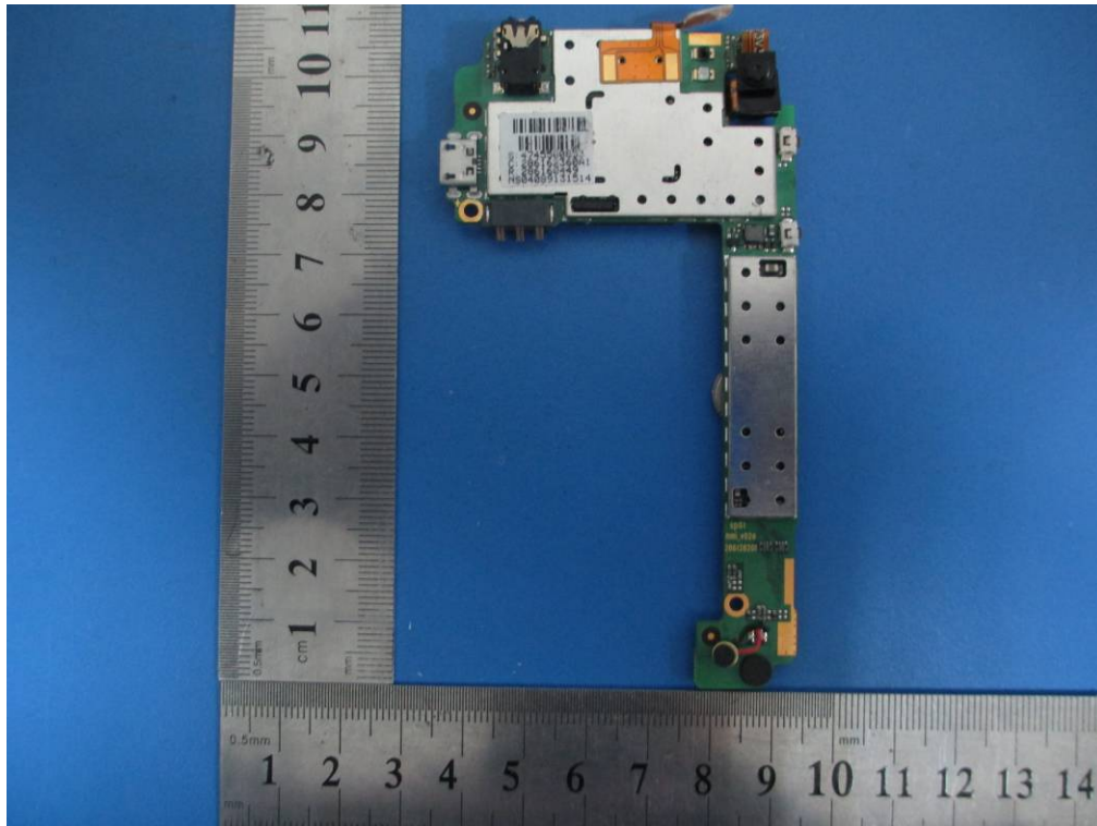
Bottom – PCB 1#
