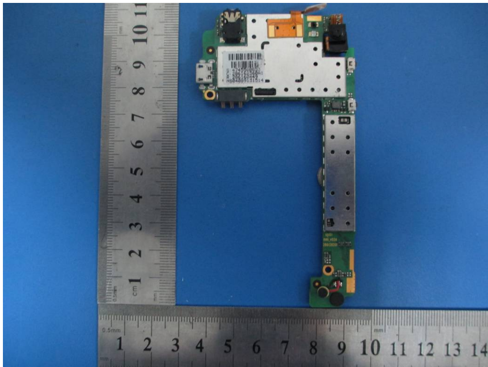
Bottom – PCB 1#
