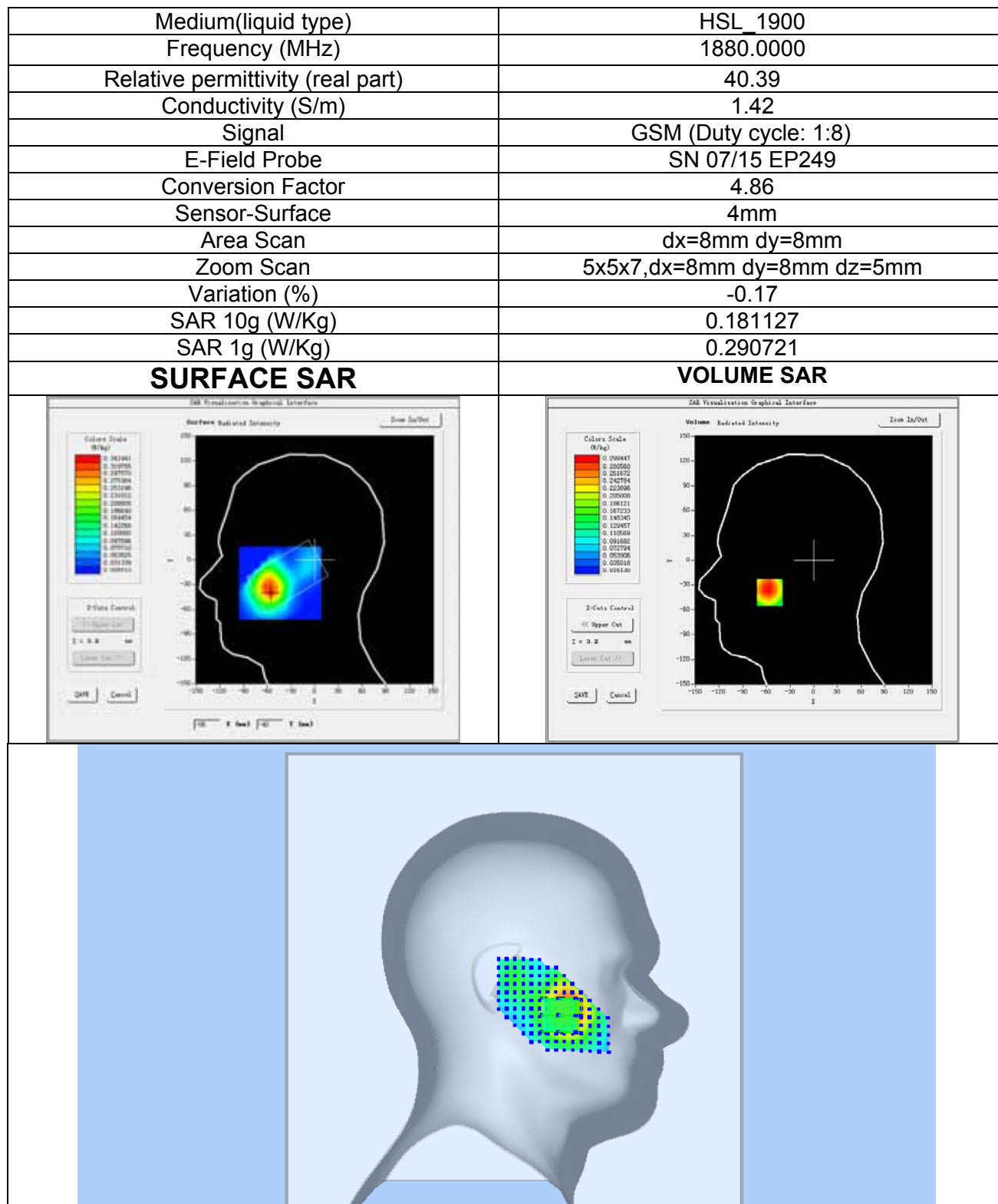
Plot 13: GSM1900, Middle channel (Left Head, Tilt) Product Description: MOBILE PHONE Test Date: Apr 14,2017
