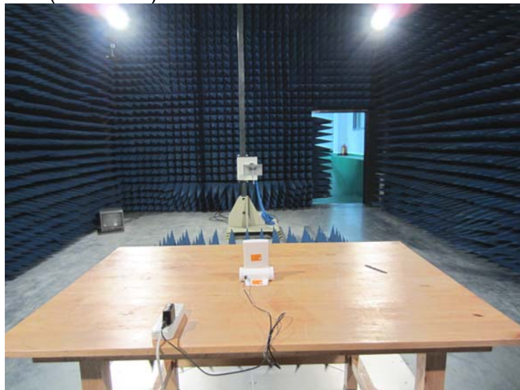
Radiated Emission(above 1G)
