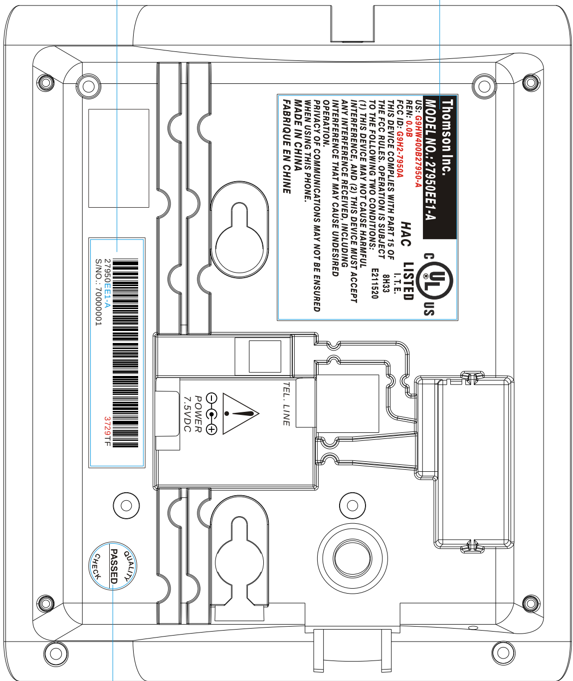
BASE S/NO. & DATE CODE LABEL SIZE: 60*14 mm
