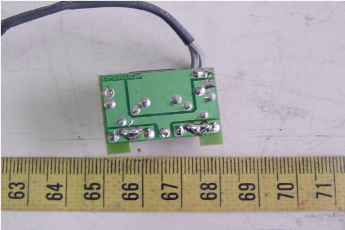
19. Solder View of Adaptor's PCB
