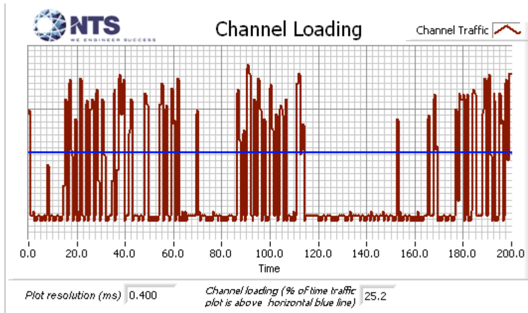
Figure 9 Channel Utilization During Testing
