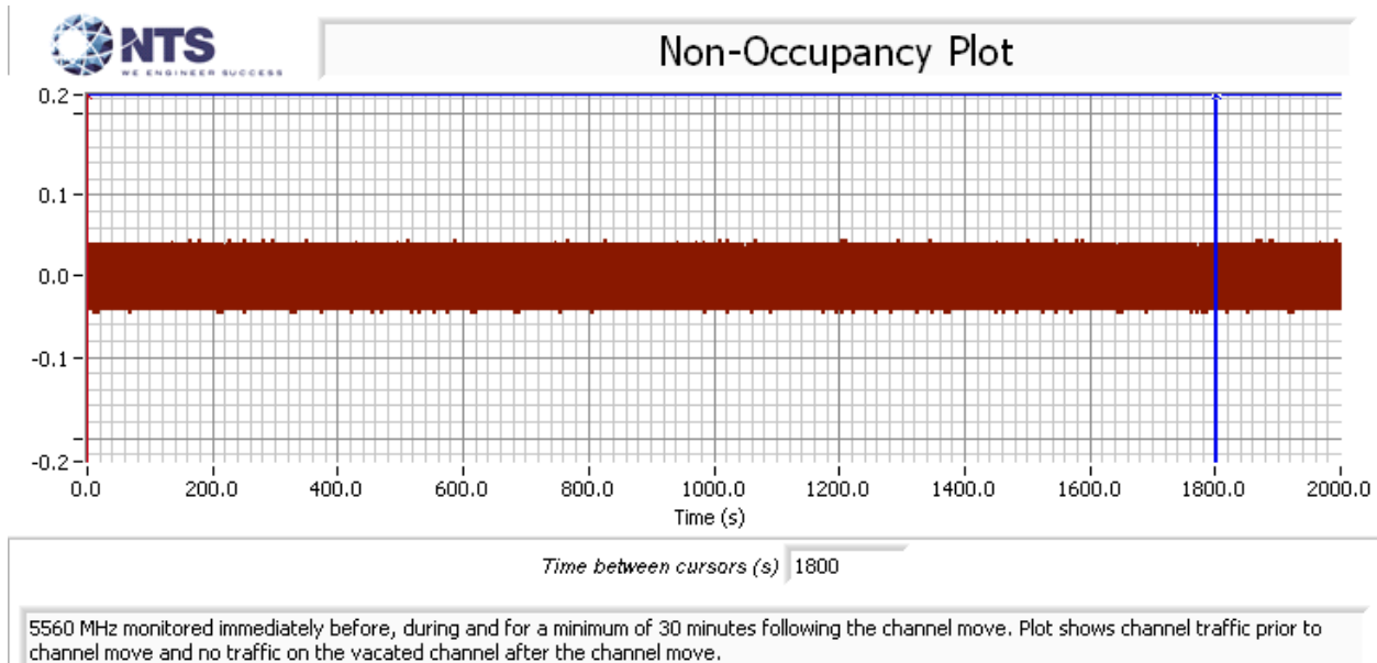
Figure 12 Radar Channel Non-occupancy Plot
