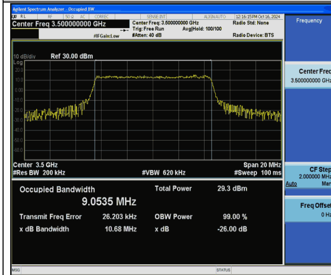
Band42(3450-3550)-10MHz-256QAM-42590-50RB#0-PASS
