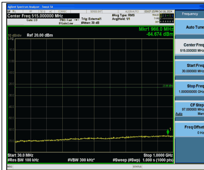
Band42(3450-3550)-20MHz-QPSK-42590-1RB#0-30~1000-PASS
