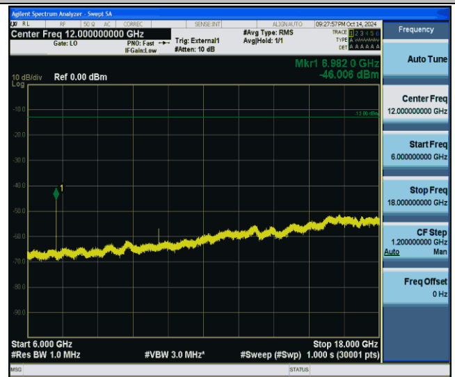
Band42(3450-3550)-20MHz-QPSK-42590-1RB#0-6000~18000-PASS
