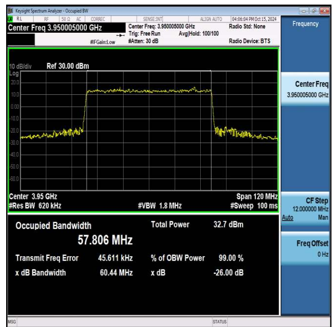
NTNV_N77-3700-3980_PC2_30_60_H_TID9_Ant1#1
