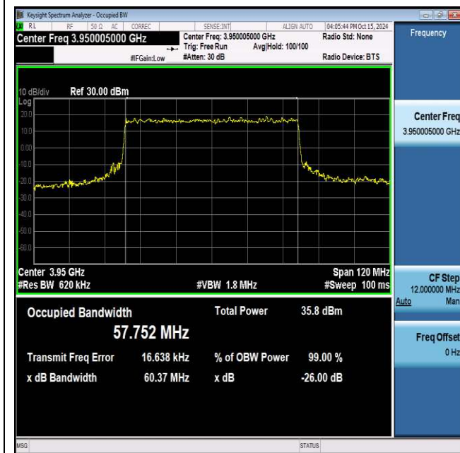
NTNV_N77-3700-3980_PC2_30_60_H_TID8_Ant1#1
