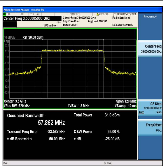
NTNV_N77-3450-3550_PC2_30_60_M_TID8_Ant1#1
