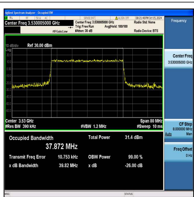
NTNV_N77-3450-3550_PC2_30_40_H_TID6_Ant1#1
