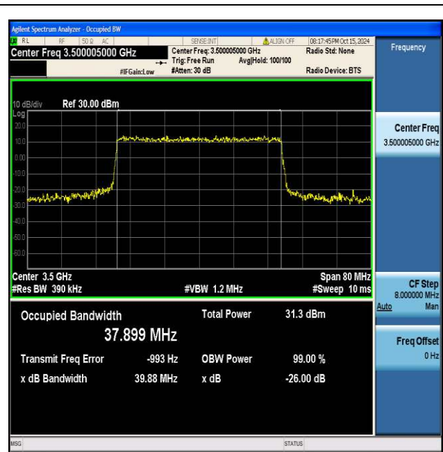
NTNV_N77-3450-3550_PC2_30_40_M_TID6_Ant1#1
