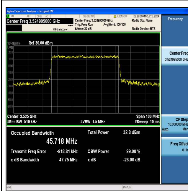
NTNV_N77-3450-3550_PC2_30_50_H_TID3_Ant1#1
