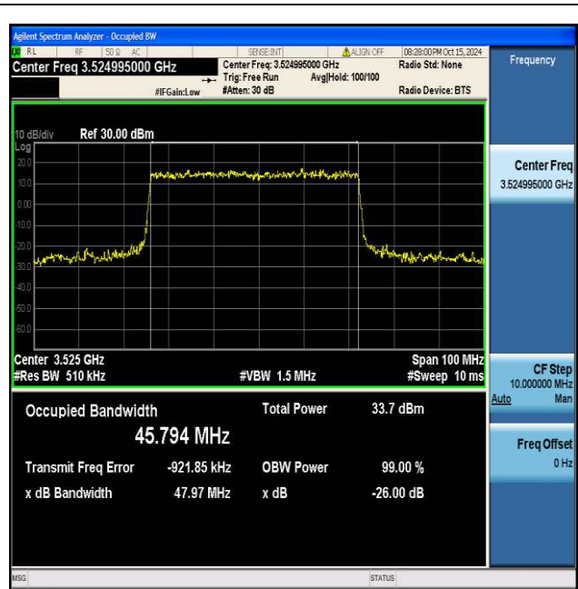
NTNV_N77-3450-3550_PC2_30_50_H_TID2_Ant1#1
