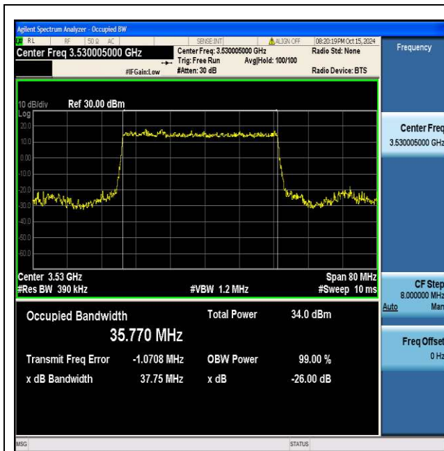
NTNV_N77-3450-3550_PC2_30_40_H_TID1_Ant1#1
