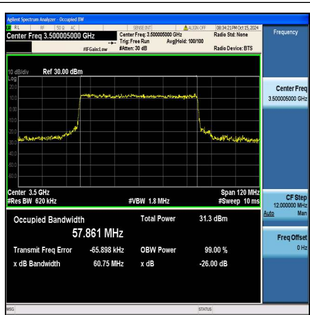
NTNV_N77-3450-3550_PC2_30_60_M_TID6_Ant1#1
