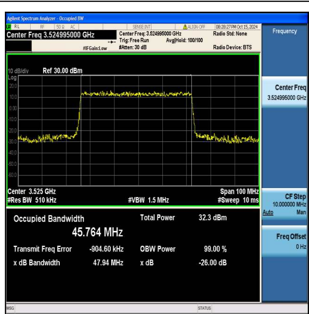
NTNV_N77-3450-3550_PC2_30_50_H_TID4_Ant1#1
