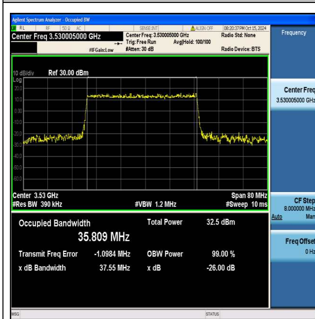
NTNV_N77-3450-3550_PC2_30_40_H_TID3_Ant1#1
