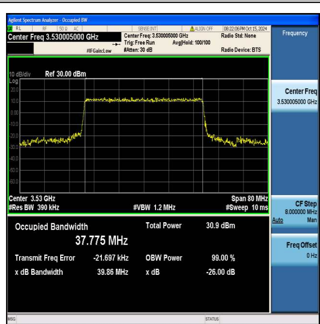
NTNV_N77-3450-3550_PC2_30_40_H_TID8_Ant1#1
