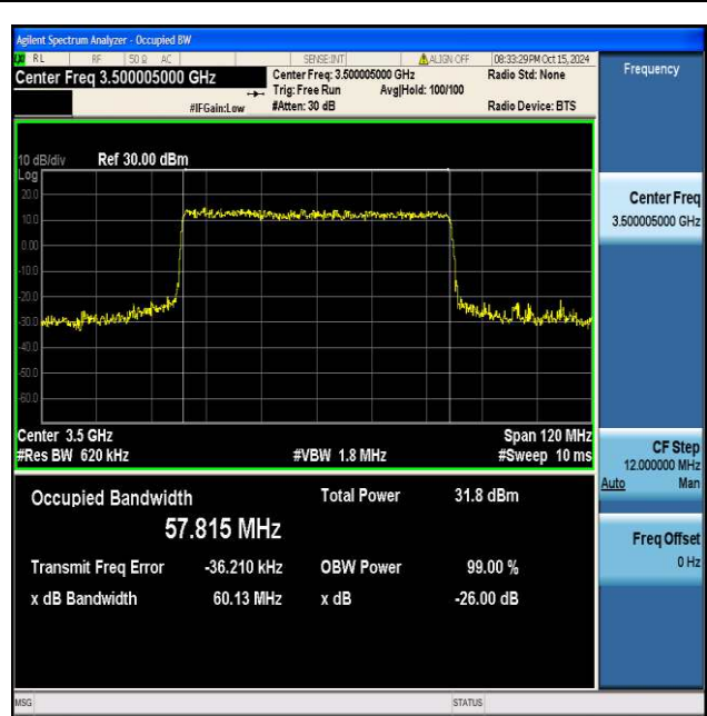
NTNV_N77-3450-3550_PC2_30_60_M_TID4_Ant1#1
