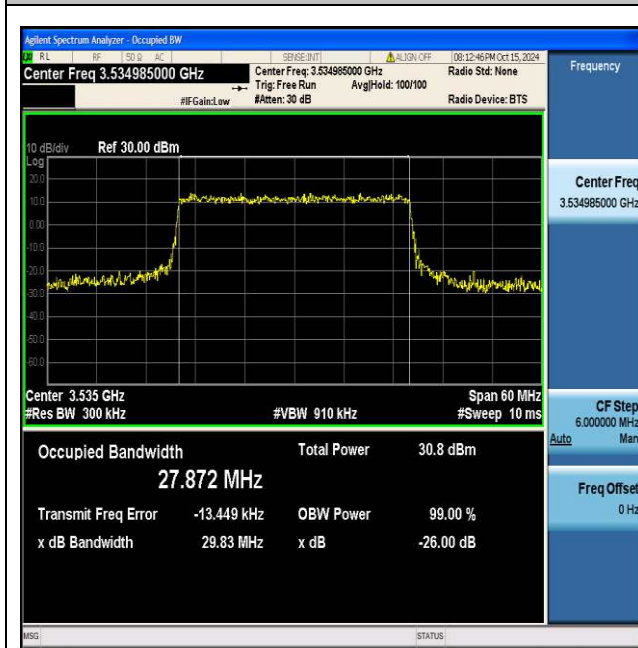
NTNV_N77-3450-3550_PC2_30_30_H_TID5_Ant1#1
