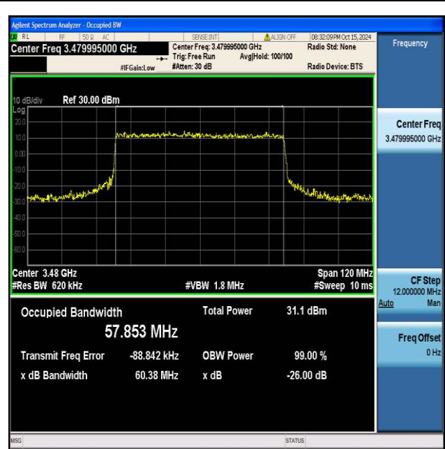
NTNV_N77-3450-3550_PC2_30_60_L_TID8_Ant1#1
