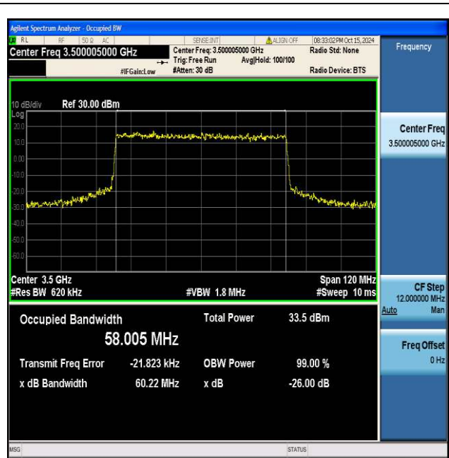
NTNV_N77-3450-3550_PC2_30_60_M_TID2_Ant1#1
