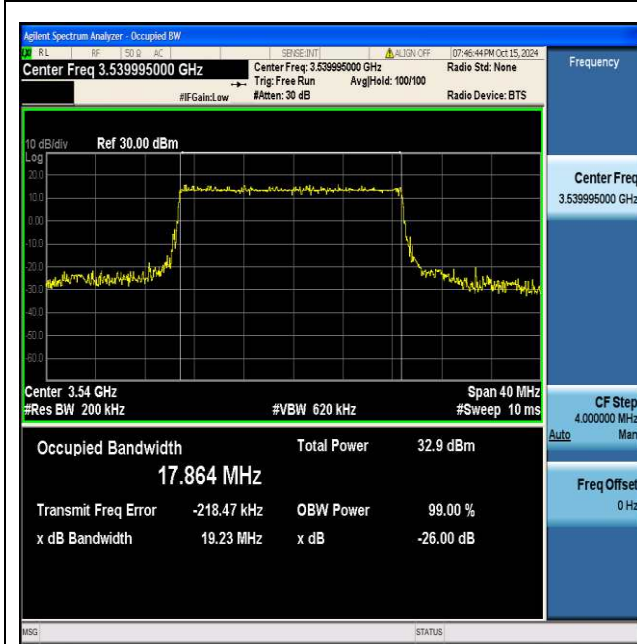
NTNV_N77-3450-3550_PC2_30_20_H_TID3_Ant1#1
