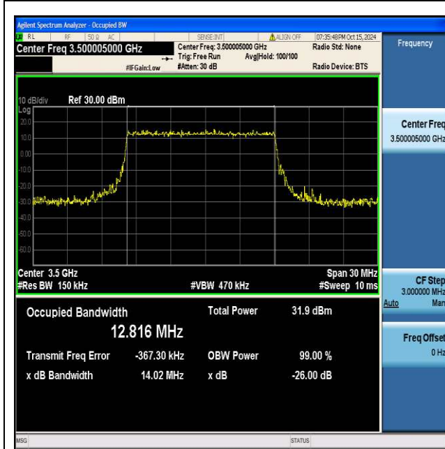
NTNV_N77-3450-3550_PC2_30_15_M_TID3_Ant1#1
