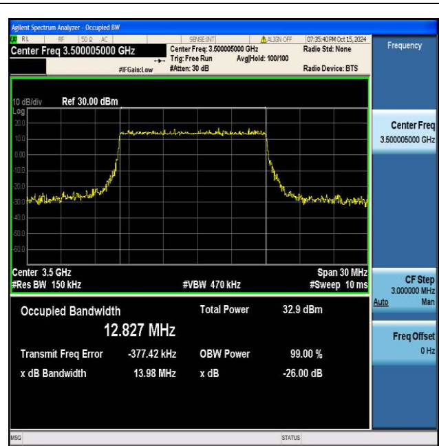
NTNV_N77-3450-3550_PC2_30_15_M_TID2_Ant1#1
