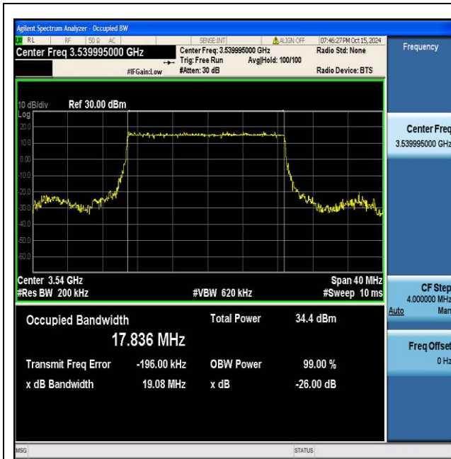
NTNV_N77-3450-3550_PC2_30_20_H_TID1_Ant1#1
