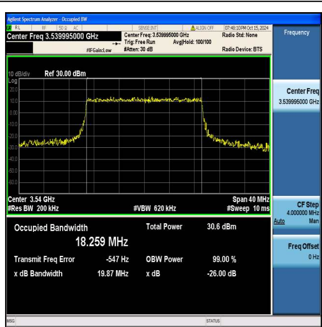
NTNV_N77-3450-3550_PC2_30_20_H_TID8_Ant1#1
