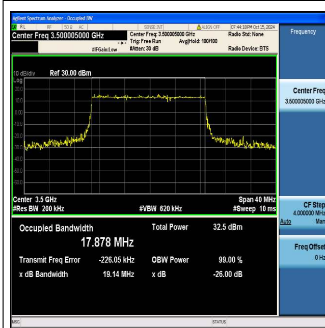
NTNV_N77-3450-3550_PC2_30_20_M_TID3_Ant1#1
