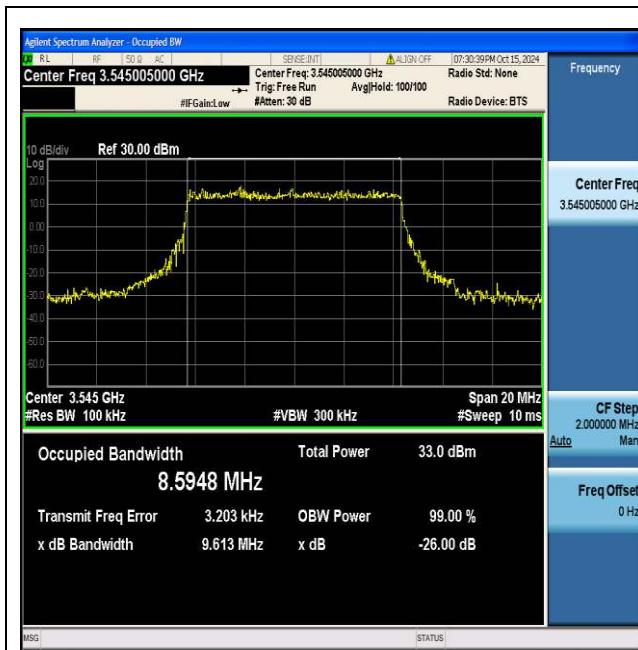
NTNV_N77-3450-3550_PC2_30_10_H_TID1_Ant1#1
