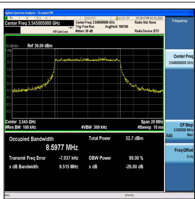
NTNV_N77-3450-3550_PC2_30_10_H_TID2_Ant1#1
