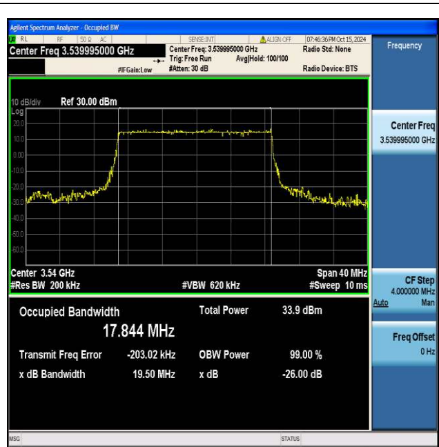
NTNV_N77-3450-3550_PC2_30_20_H_TID2_Ant1#1
