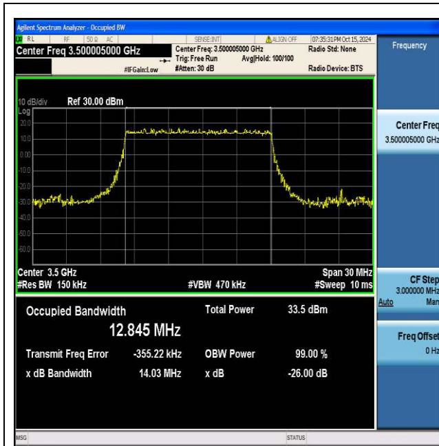
NTNV_N77-3450-3550_PC2_30_15_M_TID1_Ant1#1
