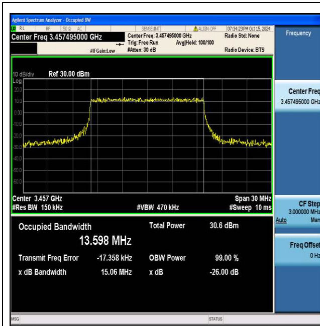
NTNV_N77-3450-3550_PC2_30_15_L_TID5_Ant1#1
