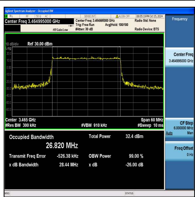
NTNV_N77-3450-3550_PC2_30_30_L_TID4_Ant1#1
