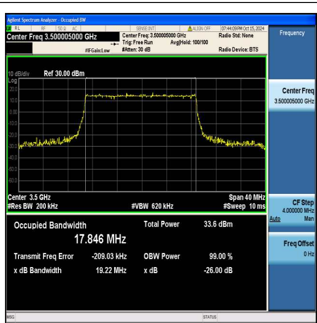
NTNV_N77-3450-3550_PC2_30_20_M_TID2_Ant1#1
