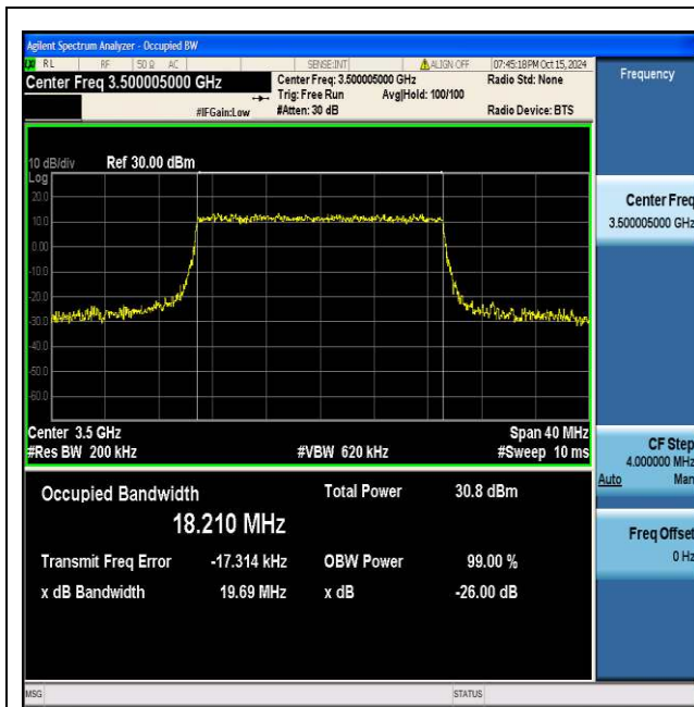
NTNV_N77-3450-3550_PC2_30_20_M_TID5_Ant1#1
