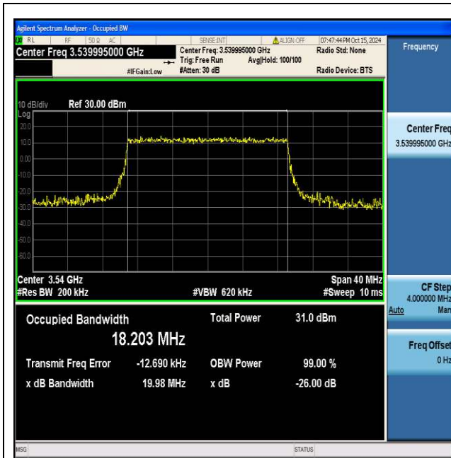
NTNV_N77-3450-3550_PC2_30_20_H_TID5_Ant1#1
