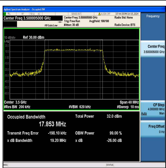
NTNV_N77-3450-3550_PC2_30_20_M_TID4_Ant1#1
