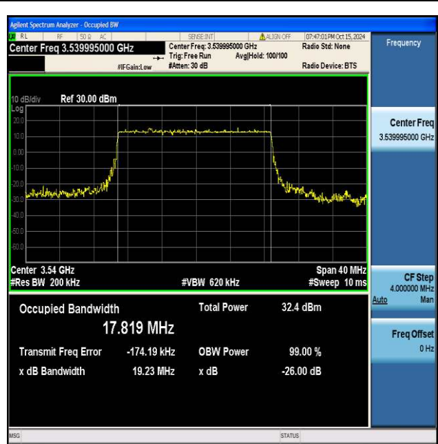
NTNV_N77-3450-3550_PC2_30_20_H_TID4_Ant1#1
