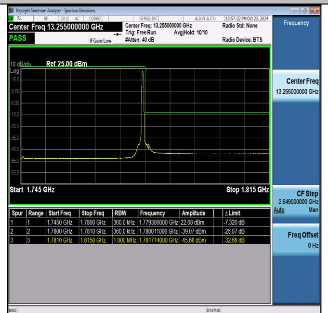
NTNV-n66-PC3-15-35-H-DFT-BPSK-Edge_1RB_Right-PASS
