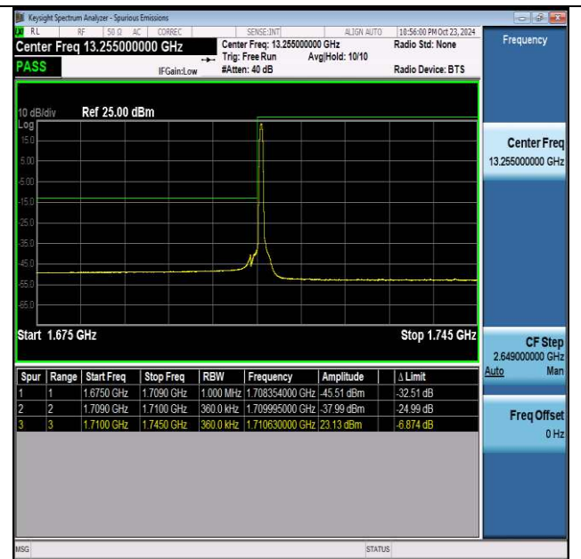
NTNV-n66-PC3-15-35-L-DFT-BPSK-Edge_1RB_Left-PASS
