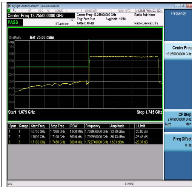
NTNV-n66-PC3-15-35-L-DFT-BPSK-Outer_Full-PASS
