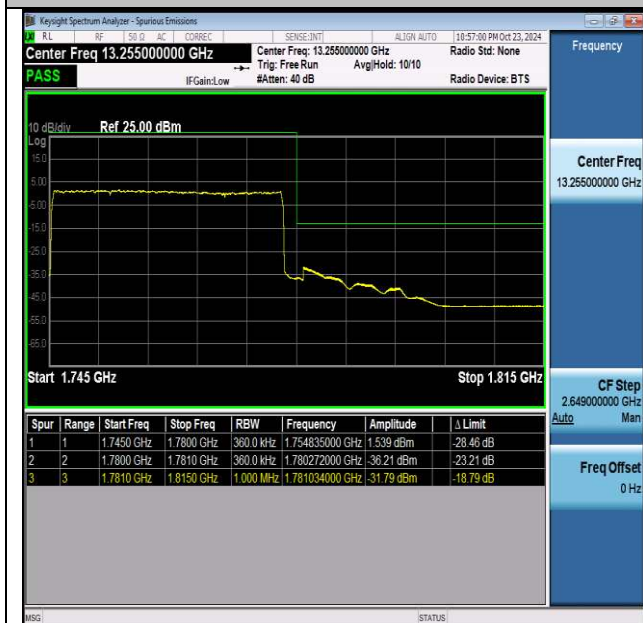
NTNV-n66-PC3-15-35-H-DFT-BPSK-Outer_Full-PASS
