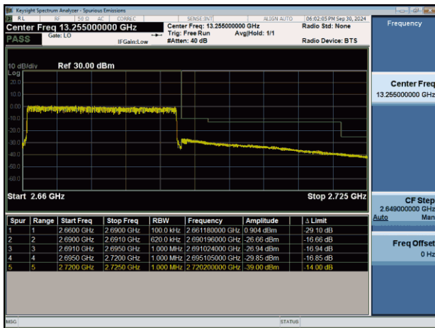
NTNV-n41-PC2-30-30-H-CP-QPSK-Outer_Full-PASS
