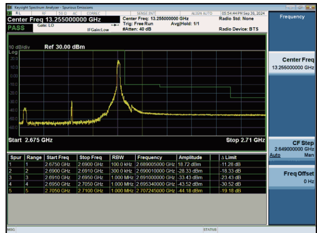
NTNV-n41-PC2-30-15-H-DFT-BPSK-Edge_1RB_Right-PASS
