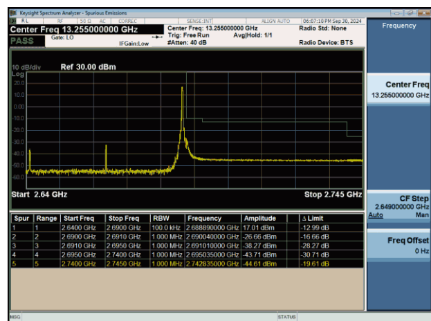
NTNV-n41-PC2-30-50-H-DFT-BPSK-Edge_1RB_Right-PASS
