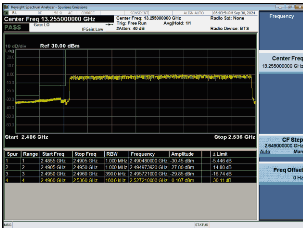
NTNV-n41-PC2-30-40-L-CP-QPSK-Outer_Full-PASS
