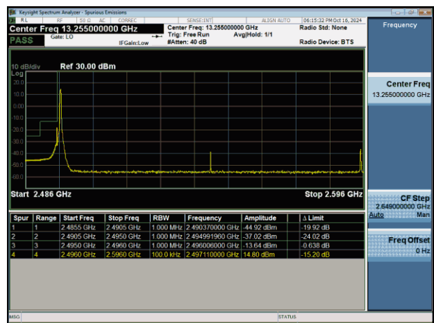
NTNV-n41-PC2-30-100-L-DFT-BPSK-Edge_1RB_Left-PASS
