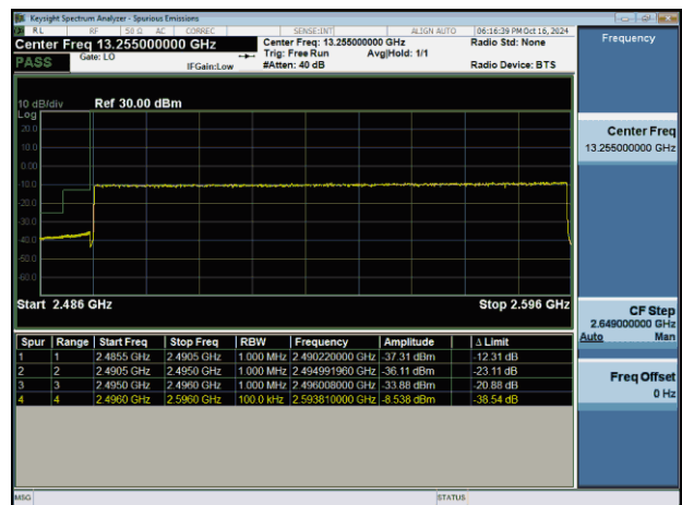
NTNV-n41-PC2-30-100-L-CP-QPSK-Outer_Full-PASS
