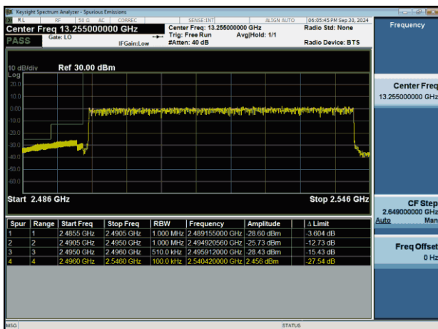
NTNV-n41-PC2-30-50-L-DFT-BPSK-Outer_Full-PASS
