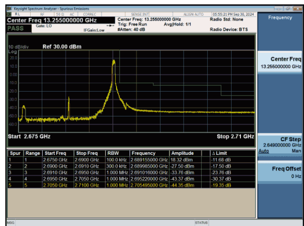
NTNV-n41-PC2-30-15-H-CP-QPSK-Edge_1RB_Right-PASS
