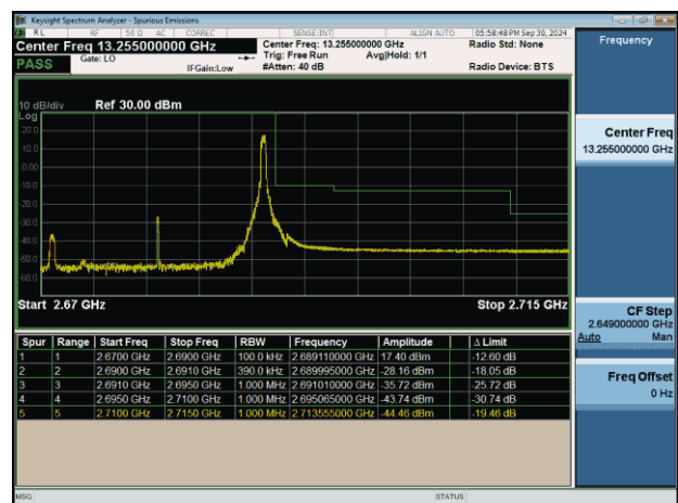
NTNV-n41-PC2-30-20-H-CP-QPSK-Edge_1RB_Right-PASS
