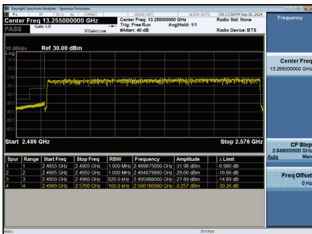
NTNV-n41-PC2-30-80-L-DFT-BPSK-Outter_Full-PASS
