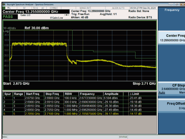
NTNV-n41-PC2-30-15-H-DFT-BPSK-Outer_Full-PASS
