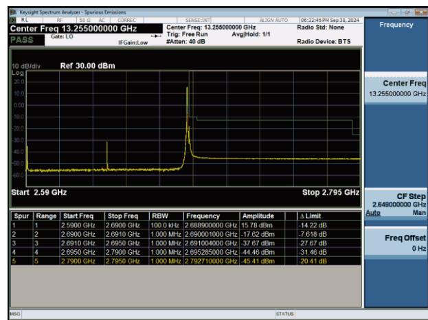
NTNV-n41-PC2-30-100-H-DFT-BPSK-Edge_1RB_Right-PASS
