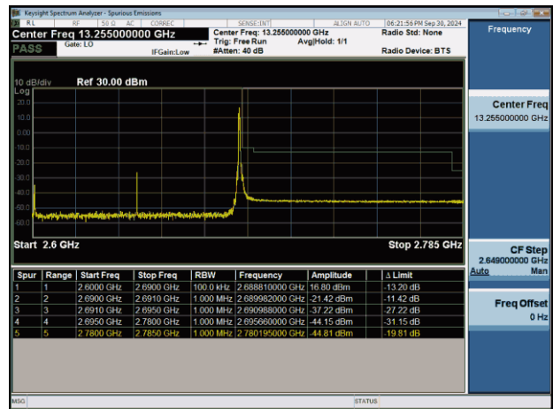
NTNV-n41-PC2-30-90-H-CP-QPSK-Edge_1RB_Right-PASS
