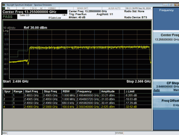
NTNV-n41-PC2-30-70-L-CP-QPSK-Outer_Full-PASS
