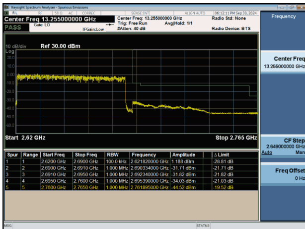
NTNV-n41-PC2-30-70-H-DFT-BPSK-Outter_Full-PASS
