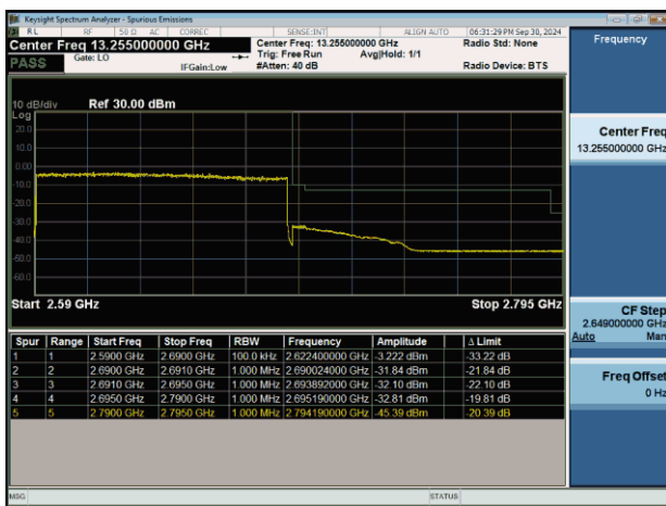
NTNV-n41-PC2-30-100-H-DFT-BPSK-Outer_Full-PASS
