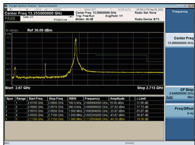
NTNV-n41-PC2-30-20-H-DFT-BPSK-Edge_1RB_Right-PASS
