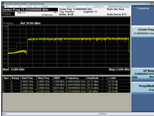
NTNV-n41-PC2-30-60-L-DFT-BPSK-Outer_Full-PASS
