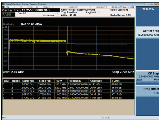
NTNV-n41-PC2-30-40-H-CP-QPSK-Outer_Full-PASS
