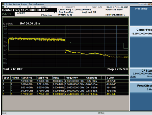
NTNV-n41-PC2-30-60-H-DFT-BPSK-Outer_Full-PASS
