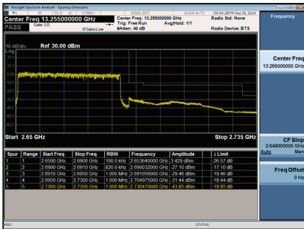
NTNV-n41-PC2-30-40-H-DFT-BPSK-Outer_Full-PASS
