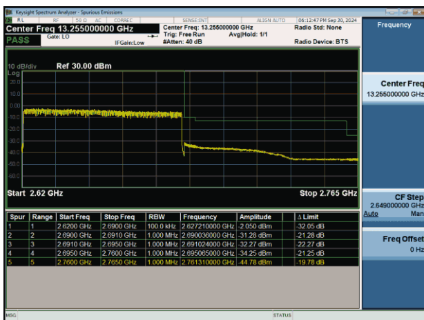
NTNV-n41-PC2-30-70-H-CP-QPSK-Outter_Full-PASS
