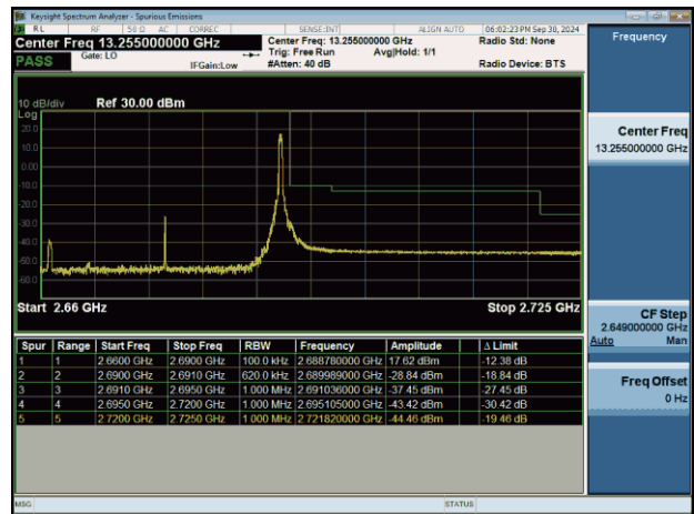
NTNV-n41-PC2-30-30-H-CP-QPSK-Edge_1RB_Right-PASS
