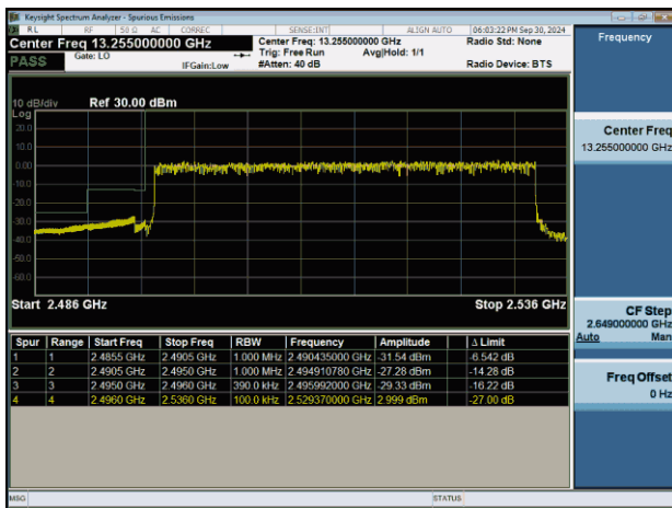
NTNV-n41-PC2-30-40-L-DFT-BPSK-Outer_Full-PASS
