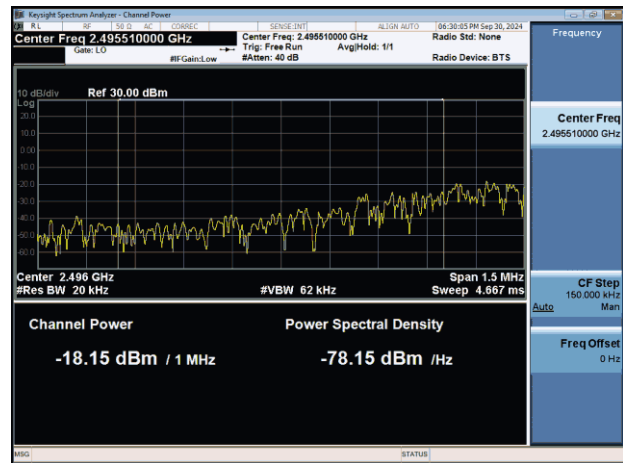
NTNV-n41-PC2-30-100-L-CP-QPSK-Edge_1RB_Left-PASS_Final1
