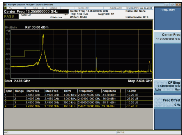
NTNV-n41-PC2-30-40-L-DFT-BPSK-Edge_1RB_Left-PASS
