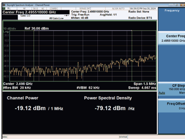
NTNV-n41-PC2-30-100-L-DFT-BPSK-Edge_1RB_Left-PASS
