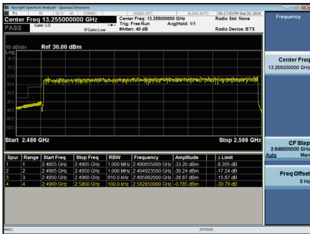
NTNV-n41-PC2-30-90-L-DFT-BPSK-Outer_Full-PASS
