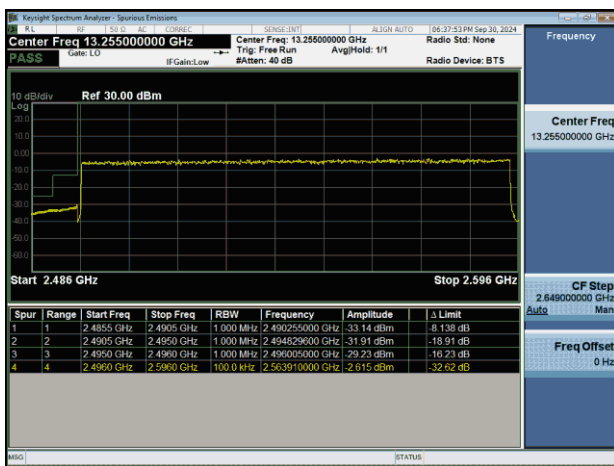
NTNV-n41-PC2-30-100-L-DFT-BPSK-Outer_Full-PASS
