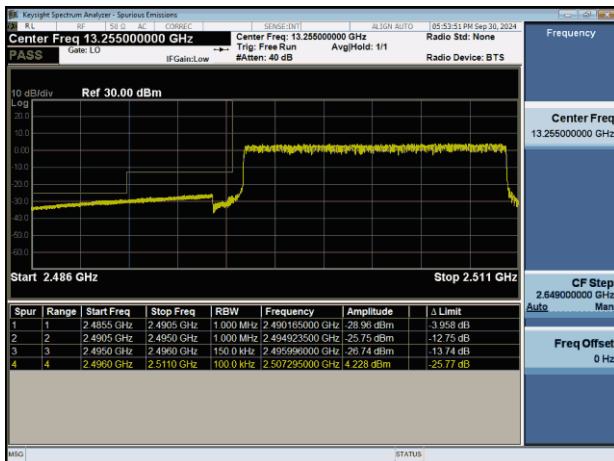
NTNV-n41-PC2-30-15-L-CP-QPSK-Outet_Full-PASS
