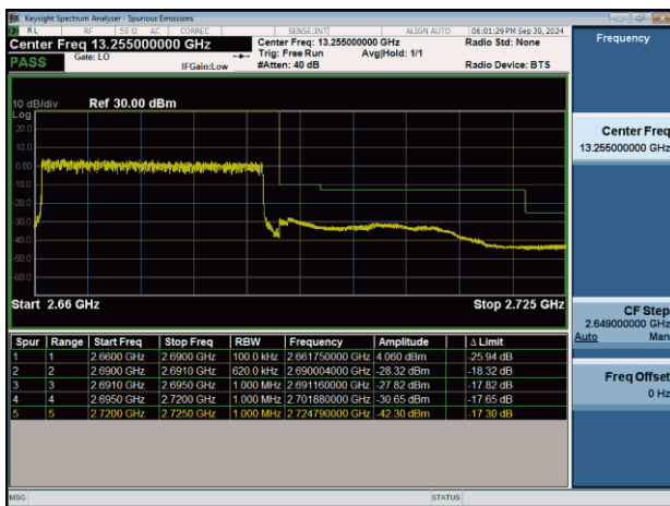
NTNV-n41-PC2-30-30-H-DFT-BPSK-Outer_Full-PASS
