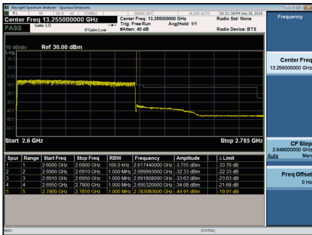
NTNV-n41-PC2-30-90-H-CP-QPSK-Outer_Full-PASS
