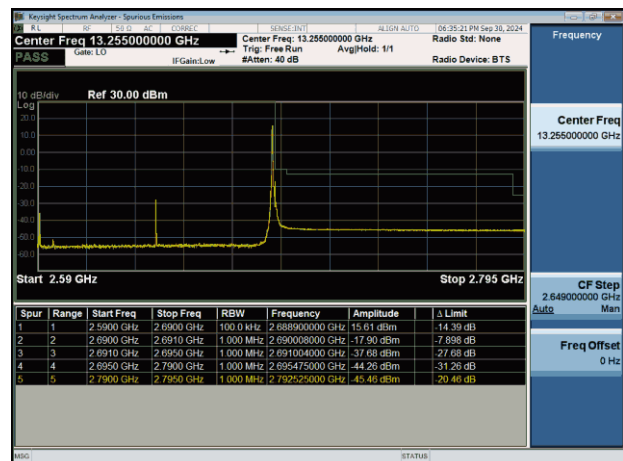
NTNV-n41-PC2-30-100-H-CP-QPSK-Edge_1RB_Right-PASS
