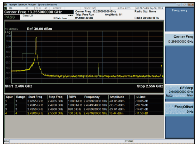
NTNV-n41-PC2-30-60-L-DFT-BPSK-Edge_1RB_Left-PASS
