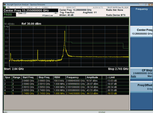
NTNV-n41-PC2-30-50-H-CP-QPSK-Edge_1RB_Right-PASS
