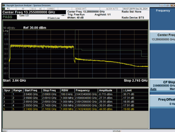
NTNV-n41-PC2-30-50-H-CP-QPSK-Outter_Full-PASS
