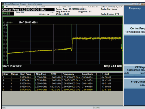
NTNV-n38-PC3-30-40-L-CP-QPSK-Outet_Full-PASS
