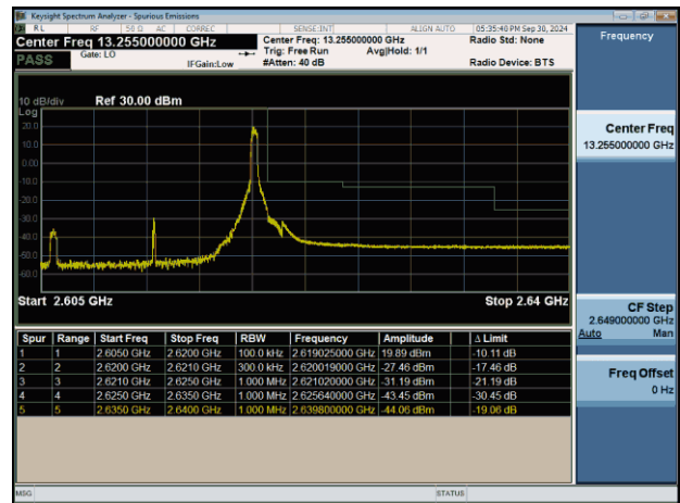
NTNV-n38-PC3-30-15-H-DFT-BPSK-Edge_1RB_Right-PASS
