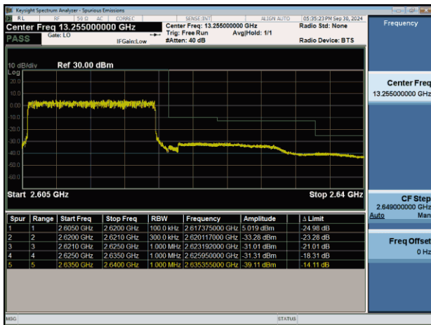
NTNV-n38-PC3-30-15-H-DFT-BPSK-Outer_Full-PASS
