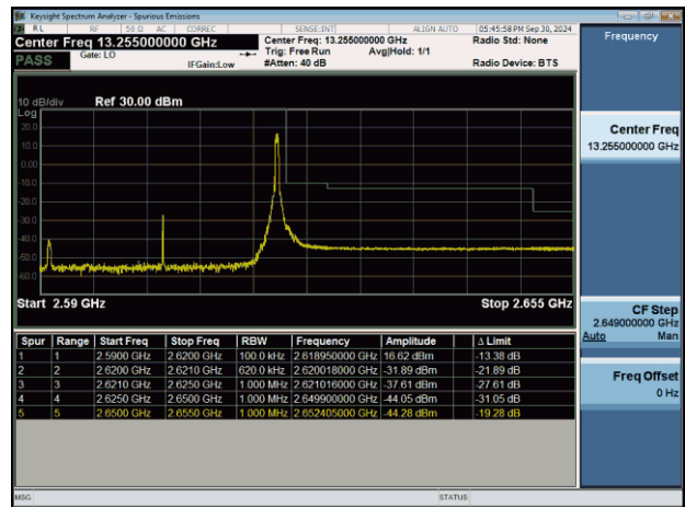
NTNV-n38-PC3-30-30-H-CP-QPSK-Edge_1RB_Right-PASS
