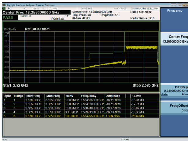
NTNV-n38-PC3-30-15-L-CP-QPSK-Outter_Full-PASS
