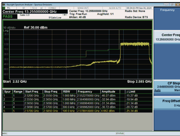
NTNV-n38-PC3-30-15-L-DFT-BPSK-Outter_Full-PASS
