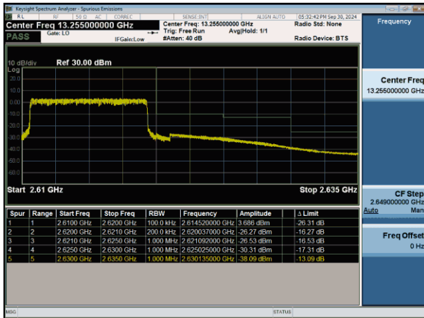
NTNV-n38-PC3-30-10-H-CP-QPSK-Outter_Full-PASS
