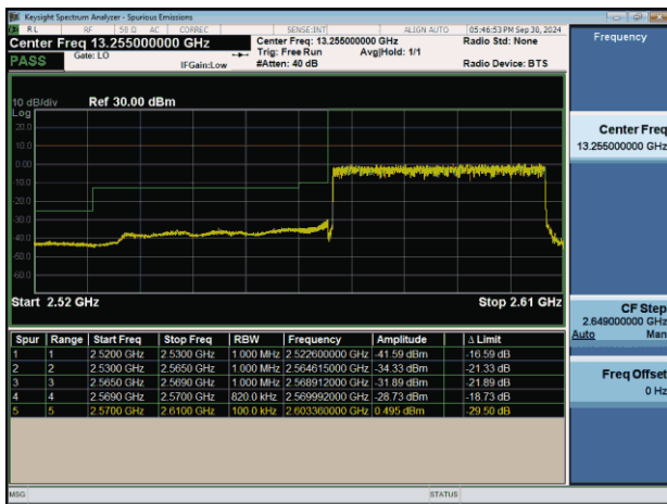
NTNV-n38-PC3-30-40-L-DFT-BPSK-Outet_Full-PASS
