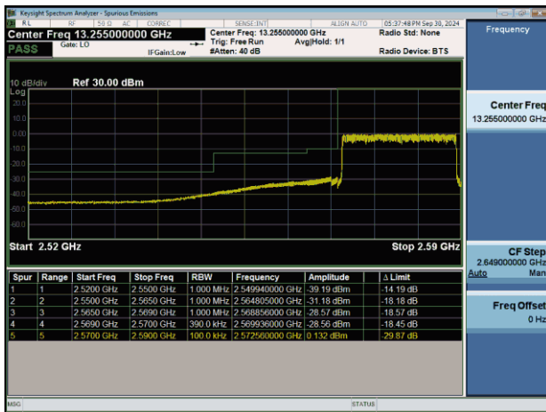
NTNV-n38-PC3-30-20-L-CP-QPSK-Outer_Full-PASS
