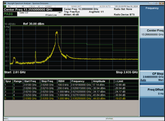
NTNV-n38-PC3-30-10-H-CP-QPSK-Edge_1RB_Right-PASS
