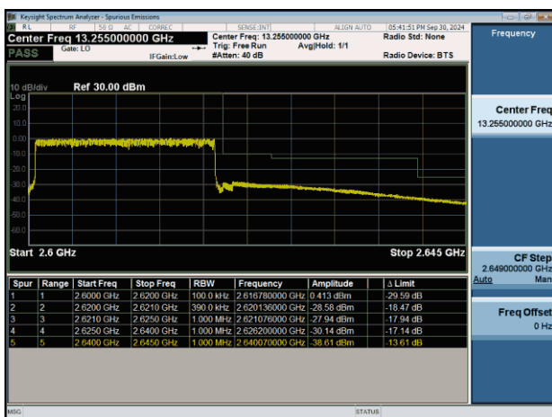
NTNV-n38-PC3-30-20-H-CP-QPSK-Outer_Full-PASS
