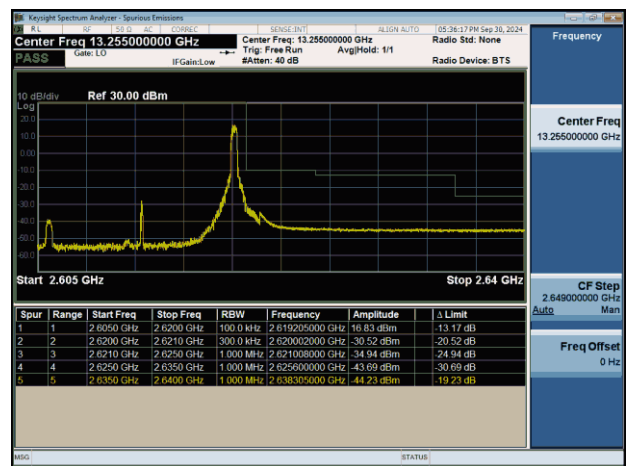
NTNV-n38-PC3-30-15-H-CP-QPSK-Edge_1RB_Right-PASS
