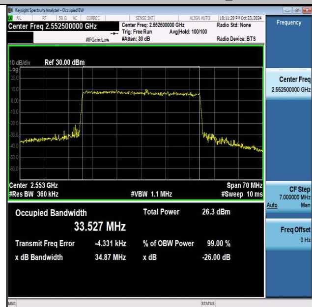
NTNV-n7-PC3-15-35-H-CP-256QAM-Outer_Full-Ant1-PASS
