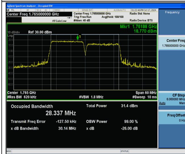
66-66-15MHz-15MHz-QPSK-QPSK-132447-132597-75RB#0-75RB#0-PASS
