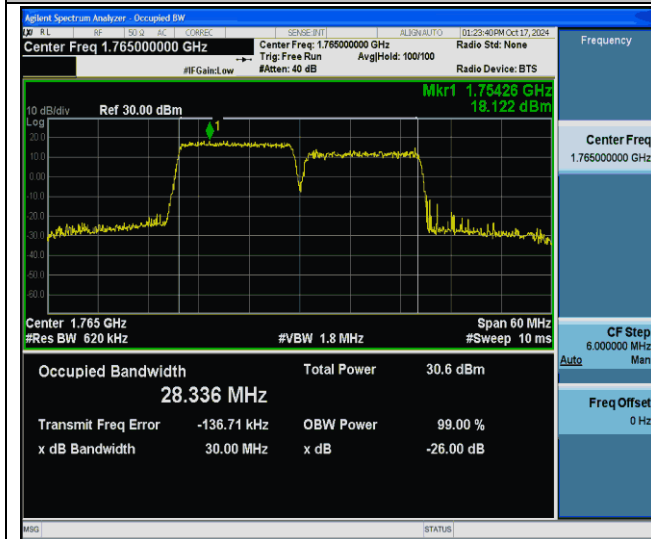
66-66-15MHz-15MHz-64QAM-64QAM-132447-132597-75RB#0-75RB#0-PASS
