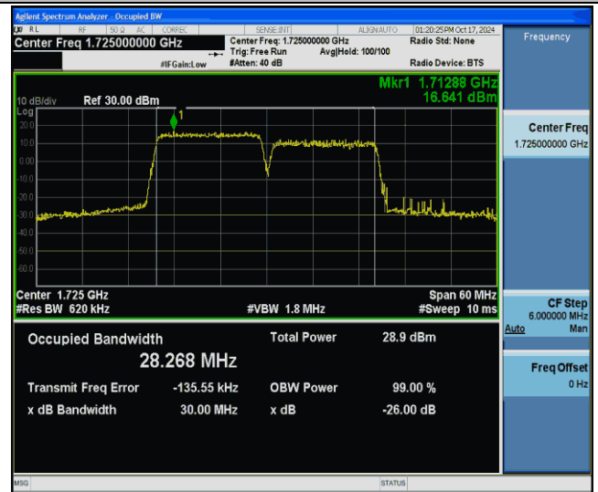
66-66-15MHz-15MHz-256QAM-256QAM-132047-132197-75RB#0-75RB#0-PASS
