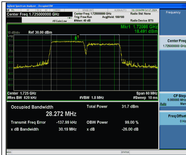
66-66-15MHz-15MHz-QPSK-QPSK-132047-132197-75RB#0-75RB#0-PASS
