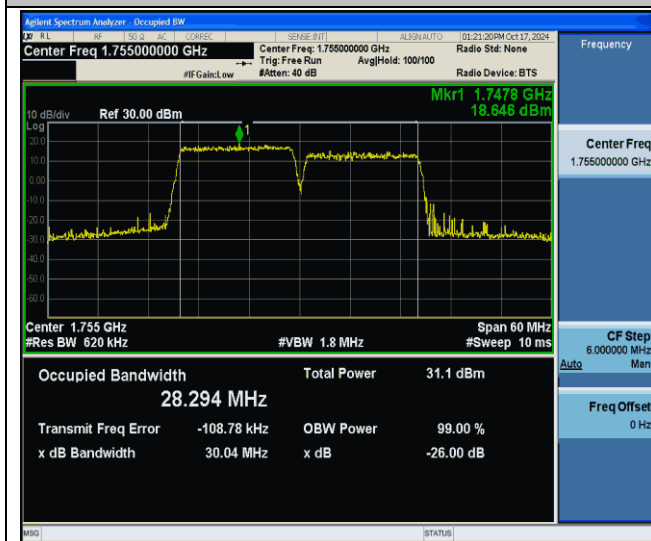
66-66-15MHz-15MHz-16QAM-16QAM-132347-132497-75RB#0-75RB#0-PASS
