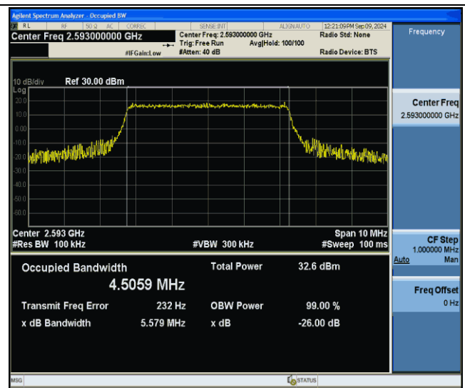
Band41-5MHz-64QAM-40620-25RB#0-PASS
