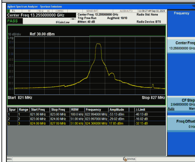
Band26(824-849)-5MHz-QPSK-26815-1RB#0-PASS
