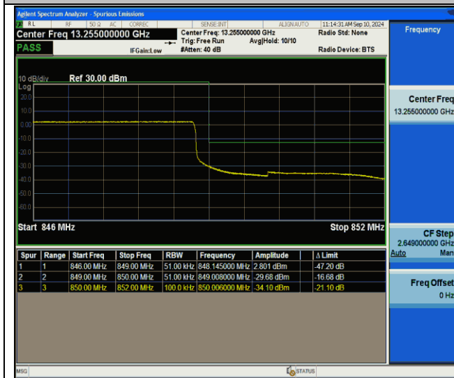
Band26(824-849)-5MHz-QPSK-27015-25RB#0-PASS
