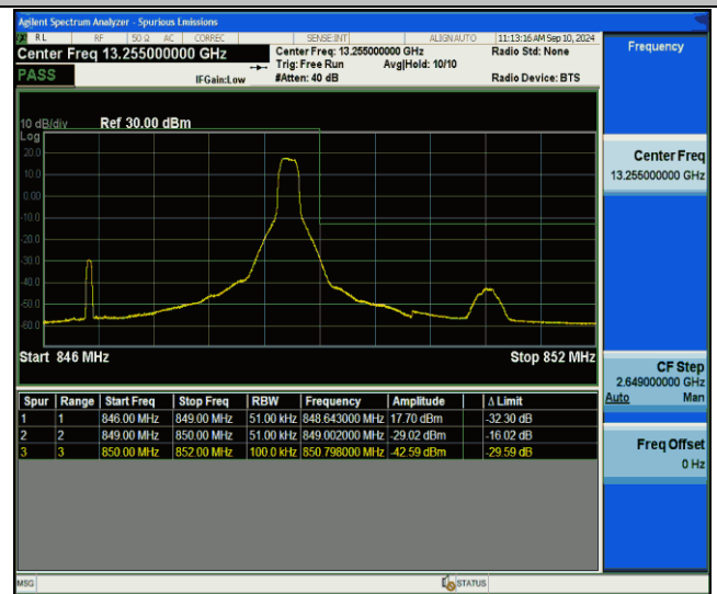
Band26(824-849)-5MHz-QPSK-27015-1RB#24-PASS
