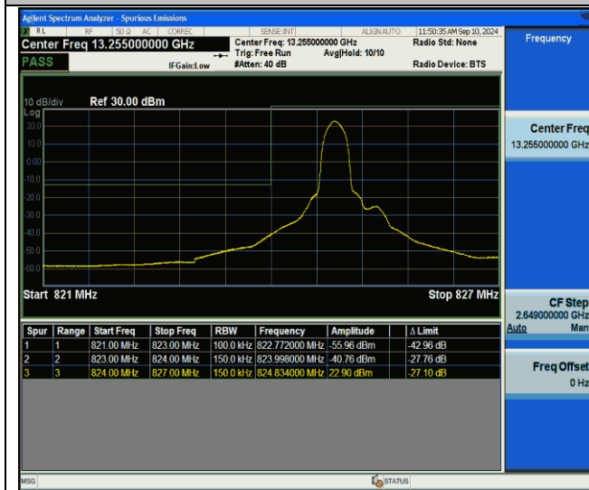
Band26(824-849)-15MHz-QPSK-26865-1RB#0-PASS
