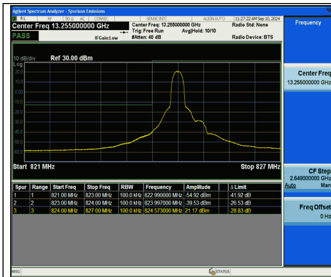
Band26(824-849)-10MHz-QPSK-26840-1RB#0-PASS
