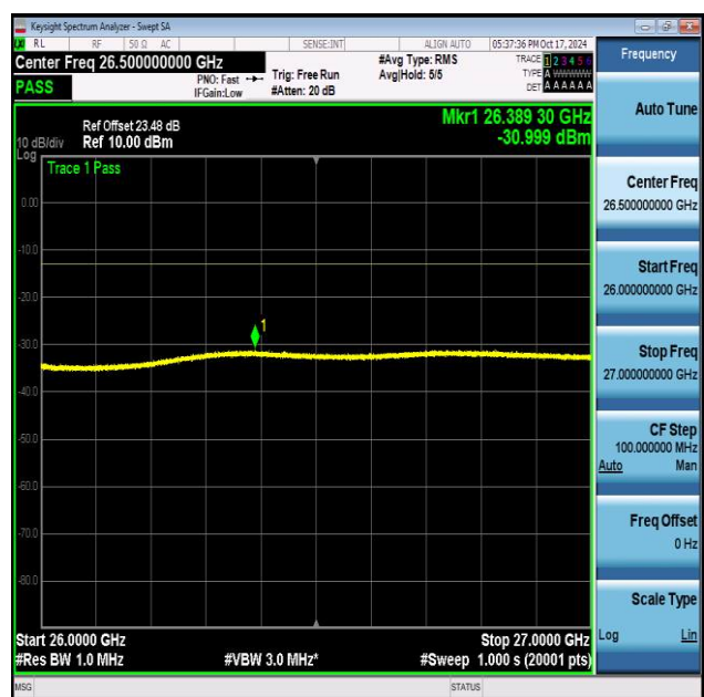
NTNV_N77-3700- 3980_PC2_30_100_H_TID1_NS_01_26000_27000_#1
