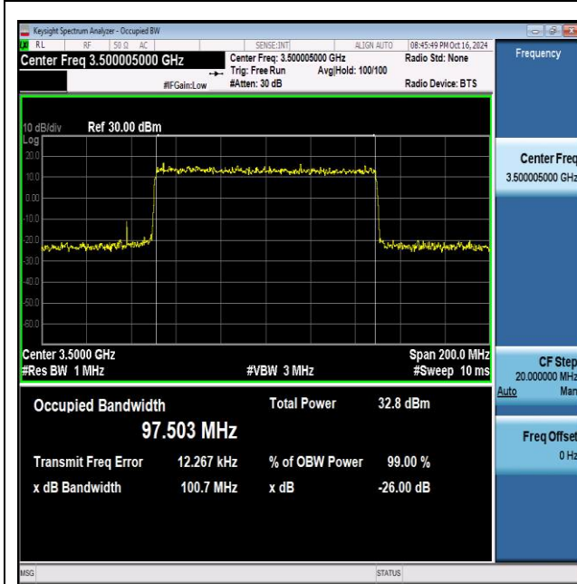
NTNV_N77-3450-3550_PC2_30_100_M_TID7_Ant1#1
