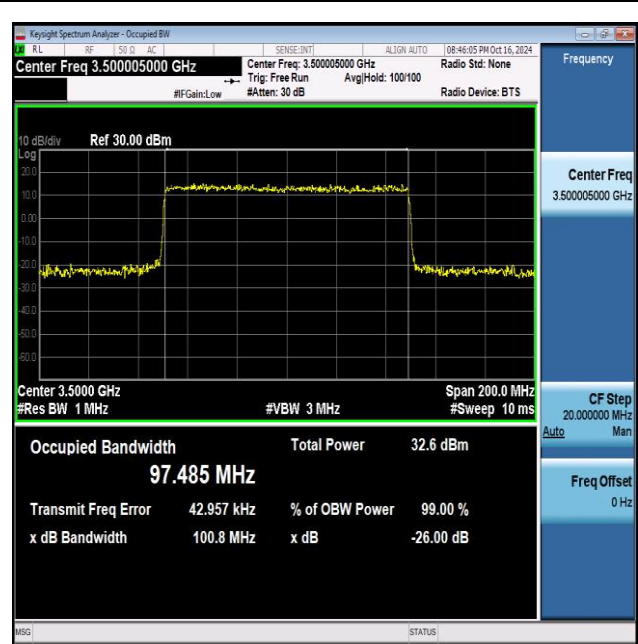
NTNV_N77-3450-3550_PC2_30_100_M_TID8_Ant1#1
