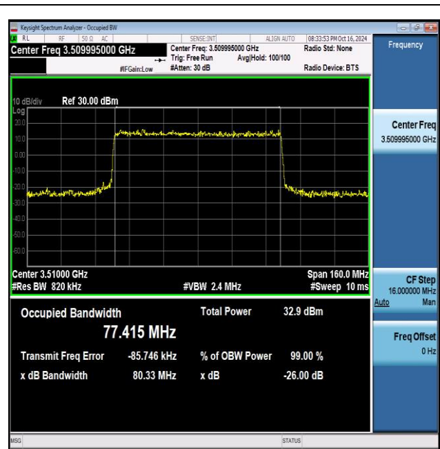
NTNV_N77-3450-3550_PC2_30_80_H_TID6_Ant1#1
