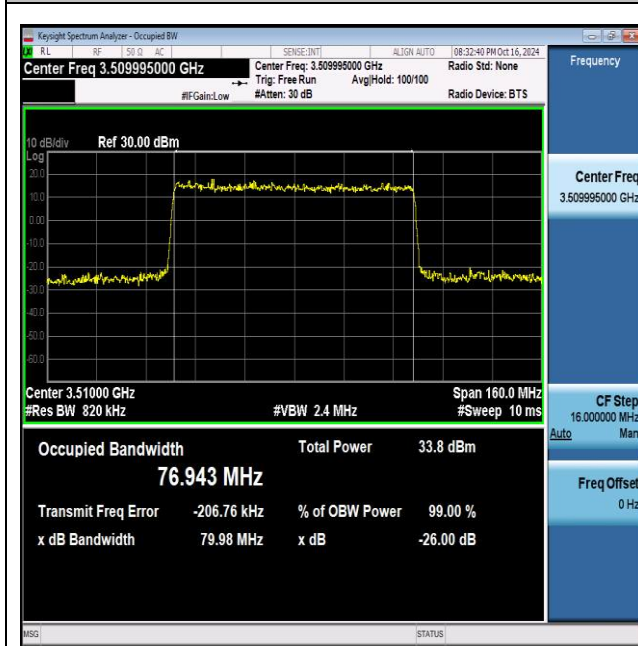
NTVN_N77-3450-3550_PC2_30_80_H_TID3_Ant1#1
