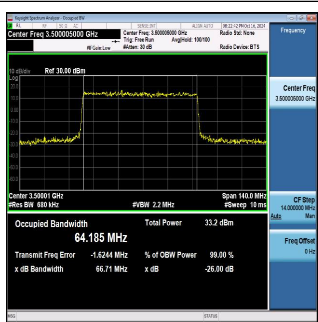
NTNV_N77-3450-3550_PC2_30_70_M_TID4_Ant1#1
