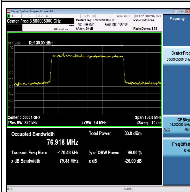
NTNV_N77-3450-3550_PC2_30_80_M_TID3_Ant1#1
