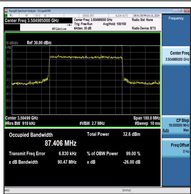
NTVN_N77-3450-3550_PC2_30_90_H_TID8_Ant1#1
