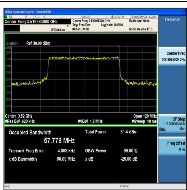
NTNV_N77-3450-3550_PC2_30_60_H_TID6_Ant1#1
