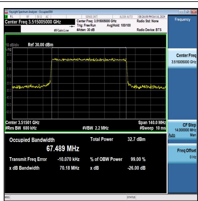
NTNV_N77-3450-3550_PC2_30_70_H_TID6_Ant1#1
