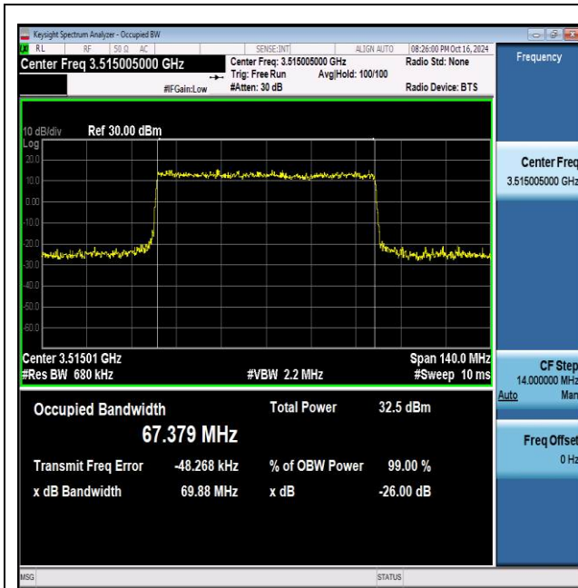
NTNV_N77-3450-3550_PC2_30_70_H_TID5_Ant1#1
