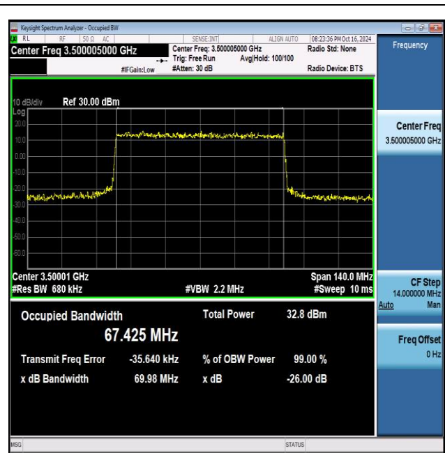
NTNV_N77-3450-3550_PC2_30_70_M_TID6_Ant1#1
