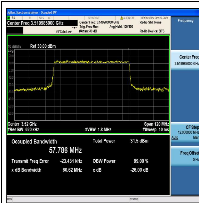
NTNV_N77-3450-3550_PC2_30_60_H_TID5_Ant1#1
