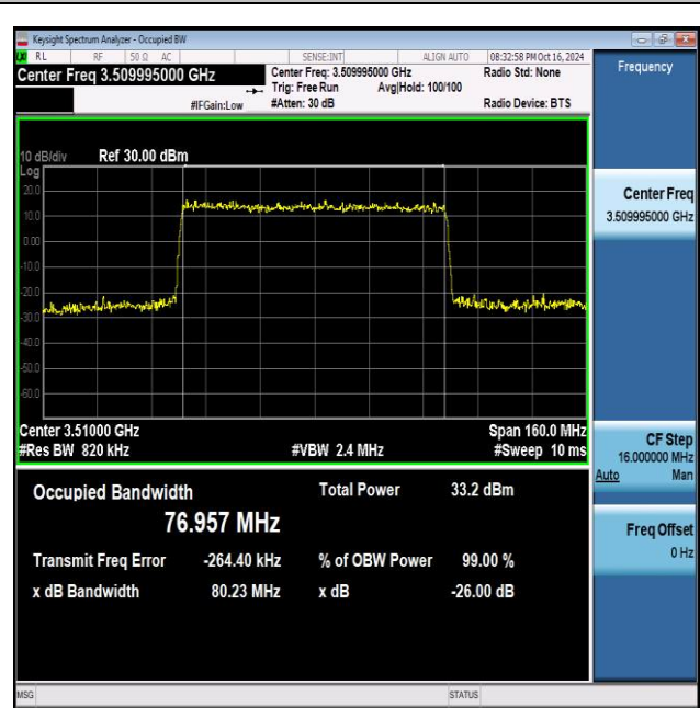
NTVN_N77-3450-3550_PC2_30_80_H_TID4_Ant1#1
