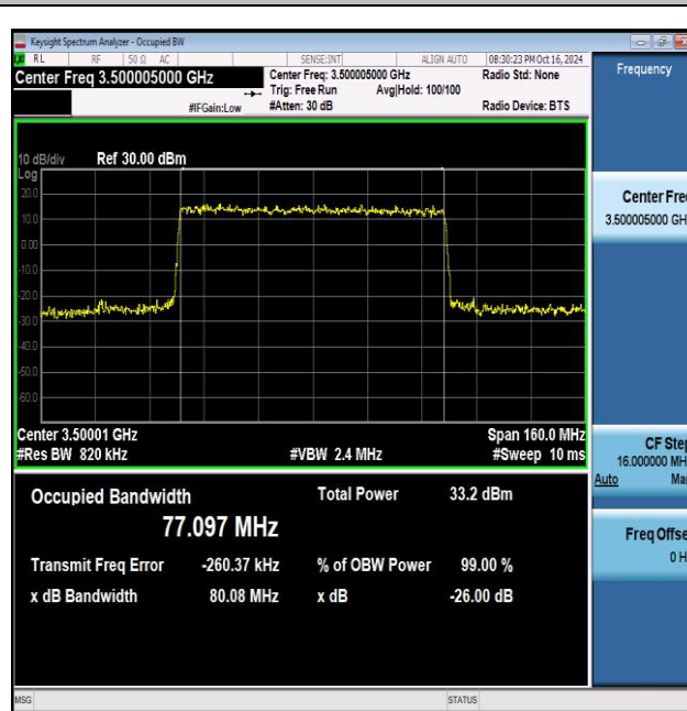
NTNV_N77-3450-3550_PC2_30_80_M_TID4_Ant1#1
