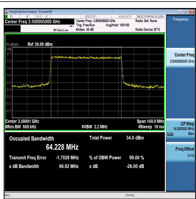
NTNV_N77-3450-3550_PC2_30_70_M_TID2_Ant1#1
