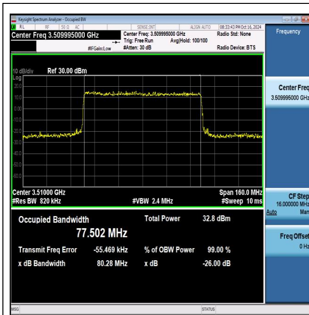
NTNV_N77-3450-3550_PC2_30_80_H_TID5_Ant1#1
