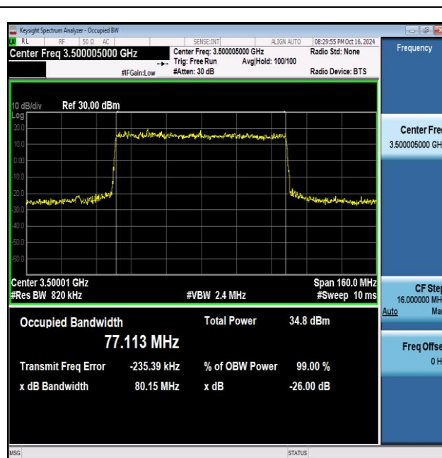
NTNV_N77-3450-3550_PC2_30_80_M_TID2_Ant1#1
