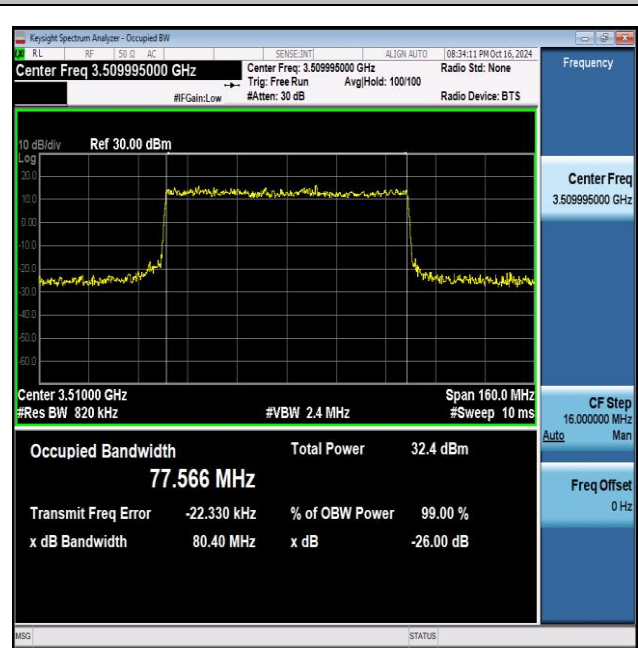
NTNV_N77-3450-3550_PC2_30_80_H_TID8_Ant1#1
