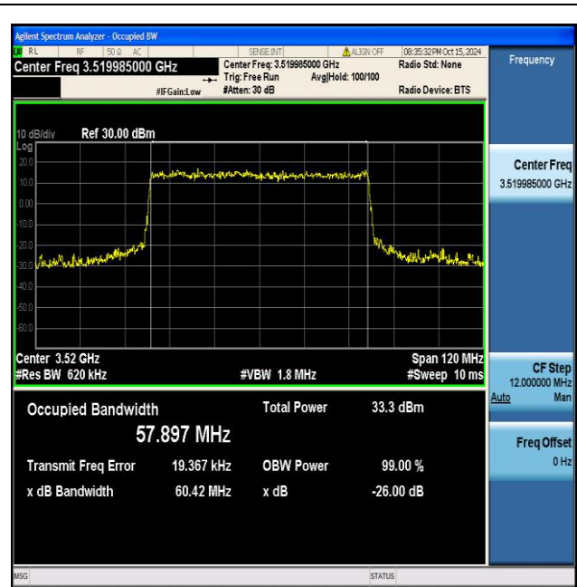
NTNV_N77-3450-3550_PC2_30_60_H_TID2_Ant1#1
