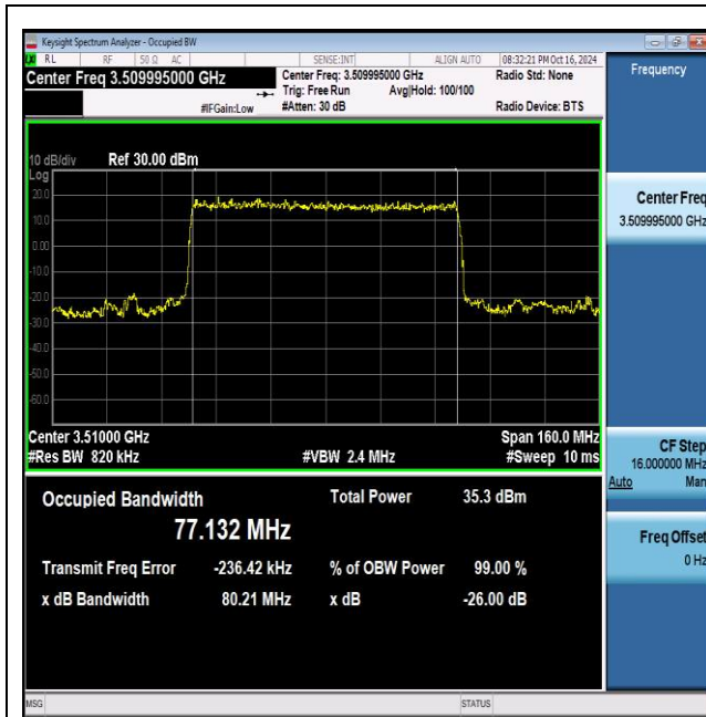
NTVN_N77-3450-3550_PC2_30_80_H_TID1_Ant1#1
