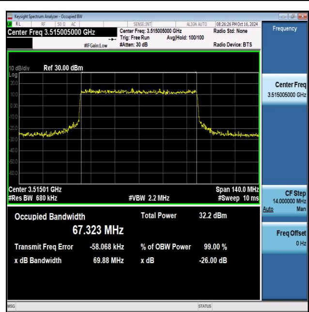
NTNV_N77-3450-3550_PC2_30_70_H_TID8_Ant1#1
