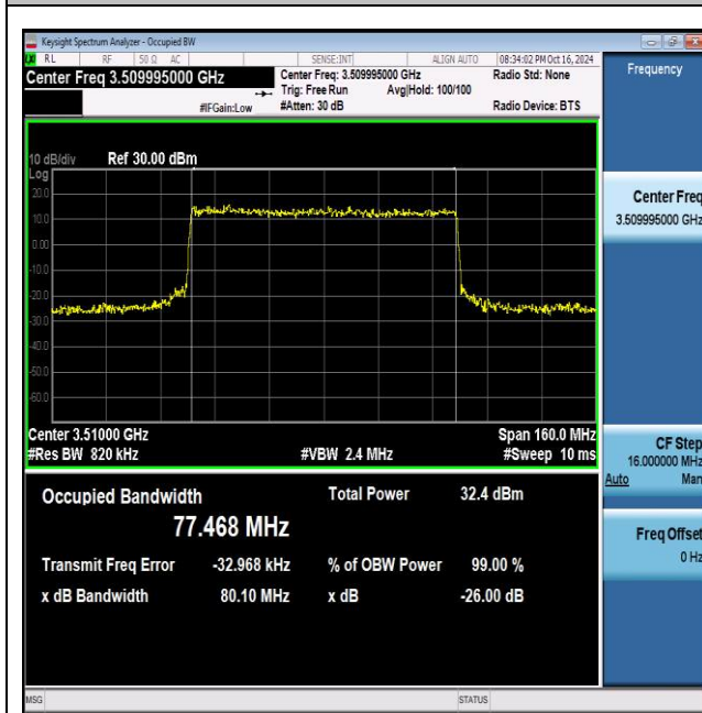
NTNV_N77-3450-3550_PC2_30_80_H_TID7_Ant1#1
