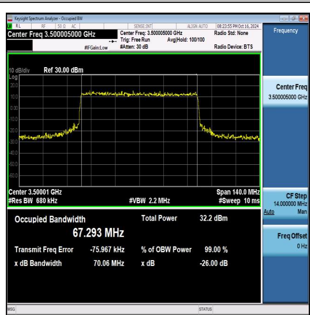
NTNV_N77-3450-3550_PC2_30_70_M_TID8_Ant1#1
