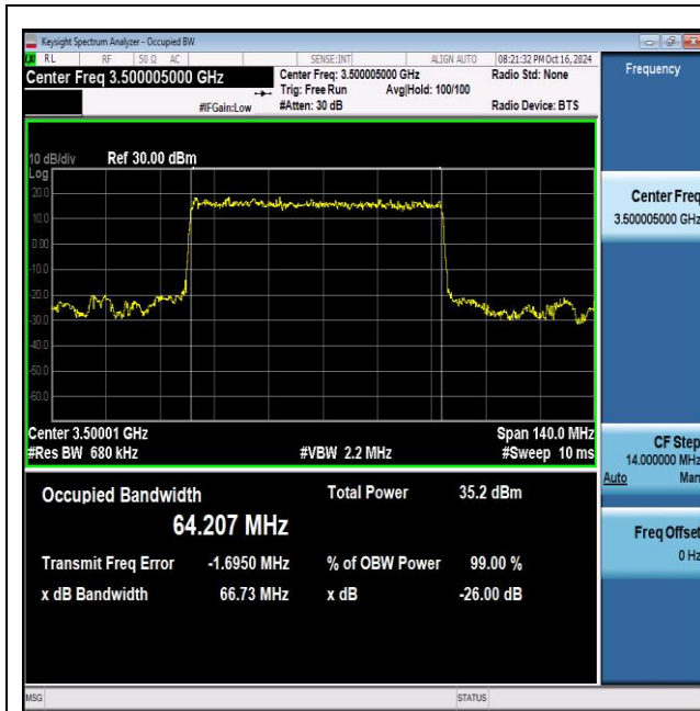
NTNV_N77-3450-3550_PC2_30_70_M_TID1_Ant1#1
