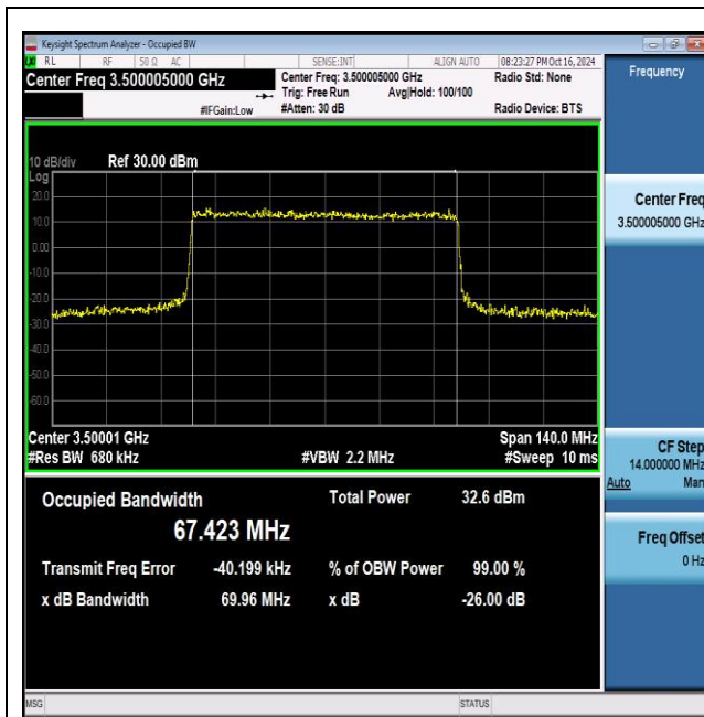
NTNV_N77-3450-3550_PC2_30_70_M_TID5_Ant1#1
