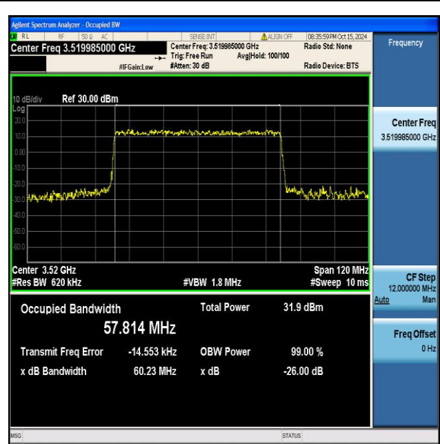
NTNV_N77-3450-3550_PC2_30_60_H_TID4_Ant1#1
