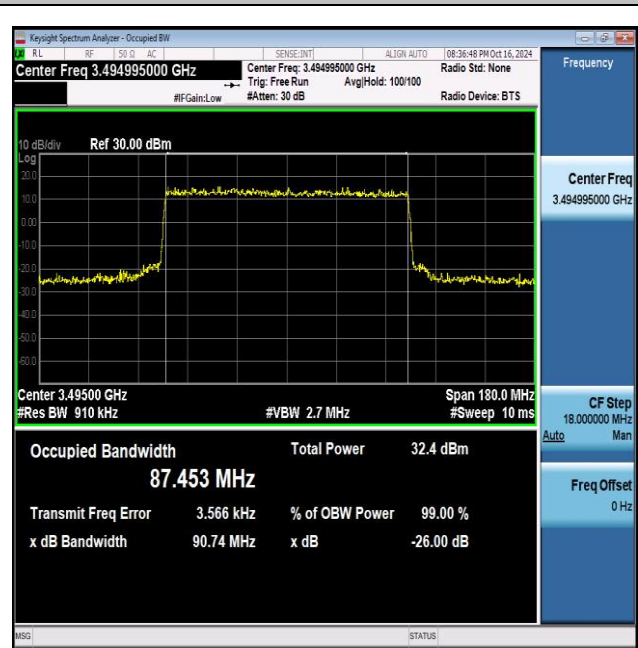
NTNV_N77-3450-3550_PC2_30_90_L_TID8_Ant1#1
