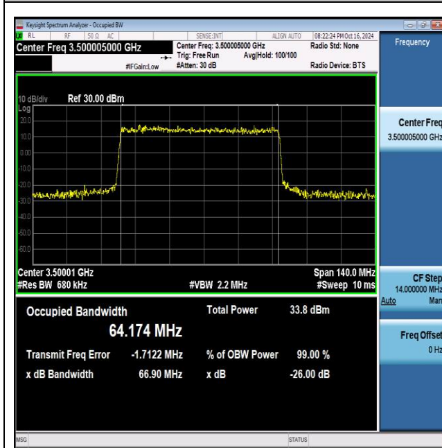
NTNV_N77-3450-3550_PC2_30_70_M_TID3_Ant1#1
