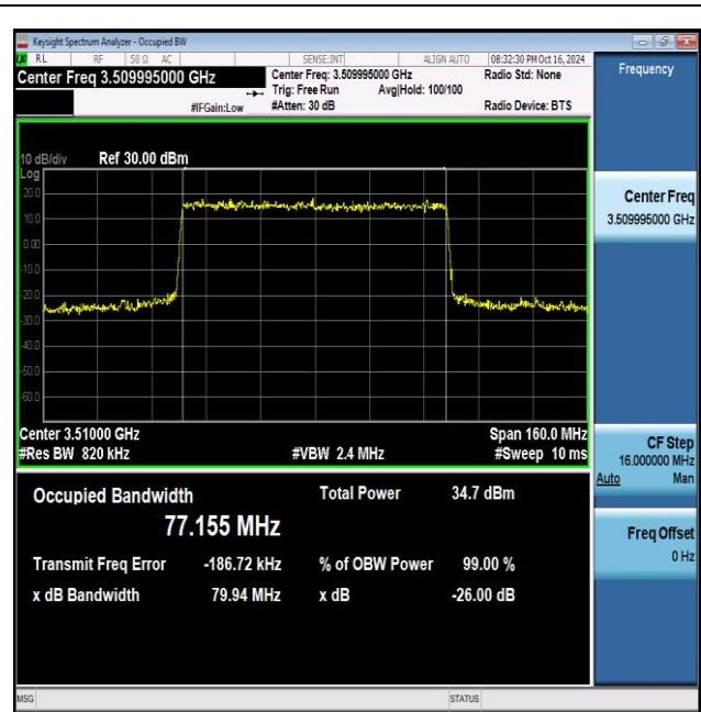
NTVN_N77-3450-3550_PC2_30_80_H_TID2_Ant1#1
