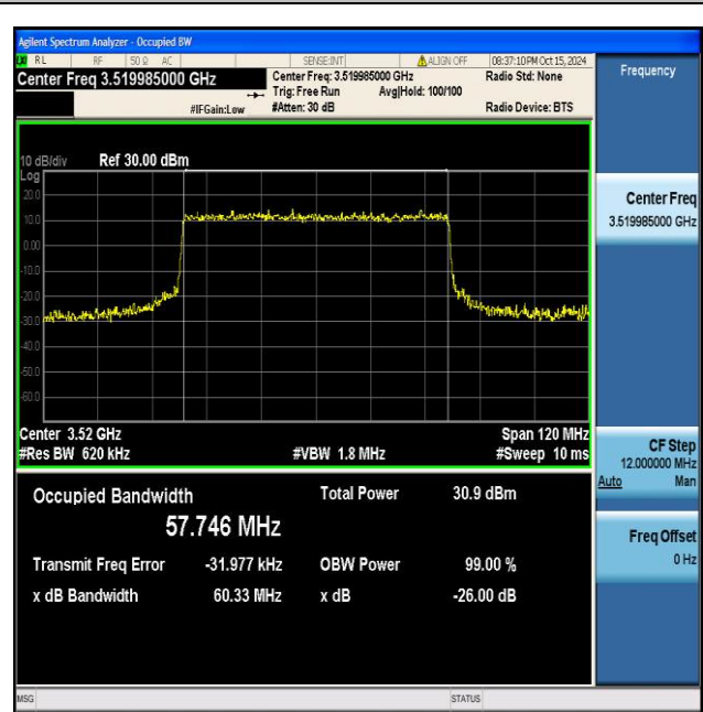
NTNV_N77-3450-3550_PC2_30_60_H_TID8_Ant1#1
