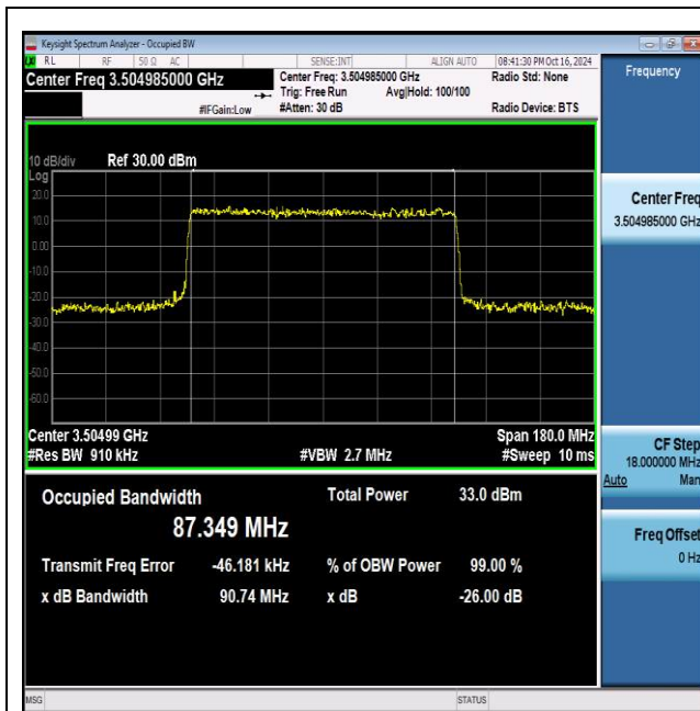
NTVN_N77-3450-3550_PC2_30_90_H_TID5_Ant1#1
