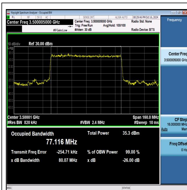
NTNV_N77-3450-3550_PC2_30_80_M_TID1_Ant1#1
