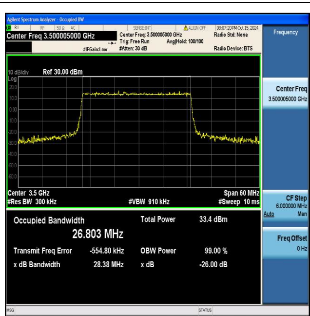
NTNV_N77-3450-3550_PC2_30_30_M_TID2_Ant1#1
