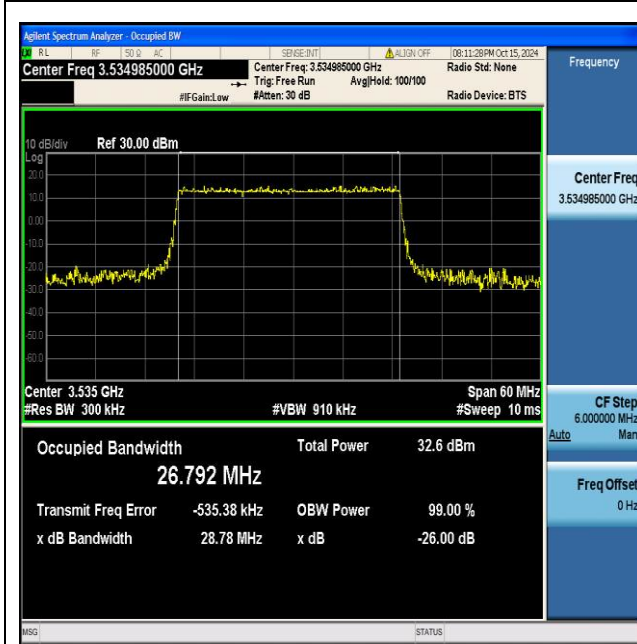
NTNV_N77-3450-3550_PC2_30_30_H_TID3_Ant1#1
