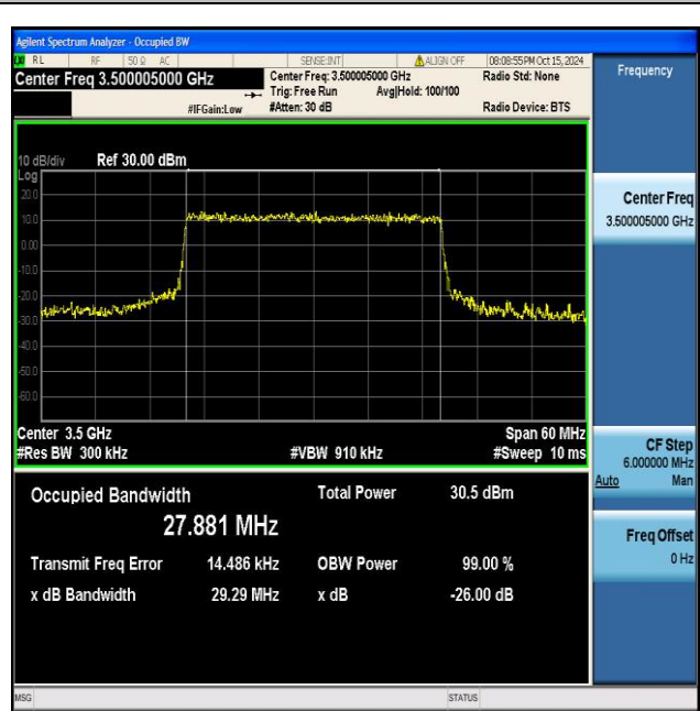
NTNV_N77-3450-3550_PC2_30_30_M_TID8_Ant1#1
