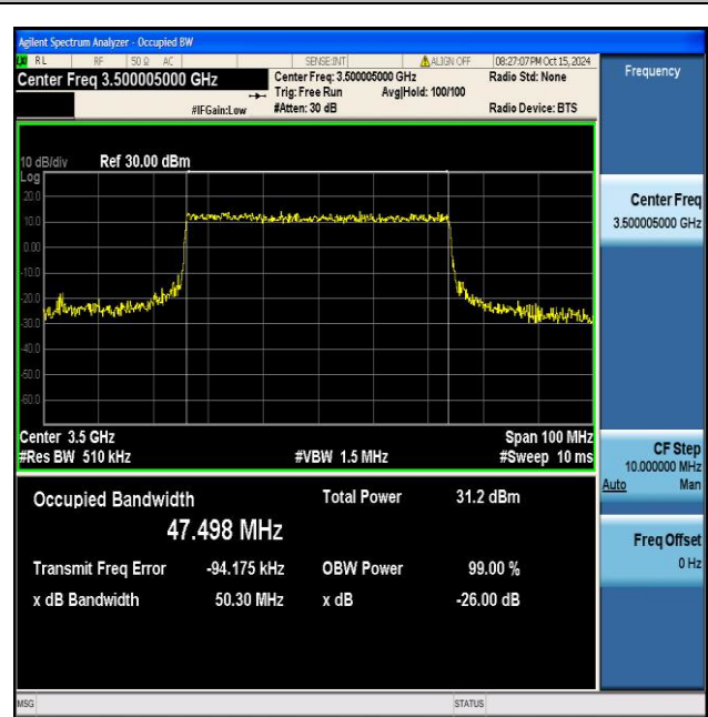
NTNV_N77-3450-3550_PC2_30_50_M_TID8_Ant1#1
