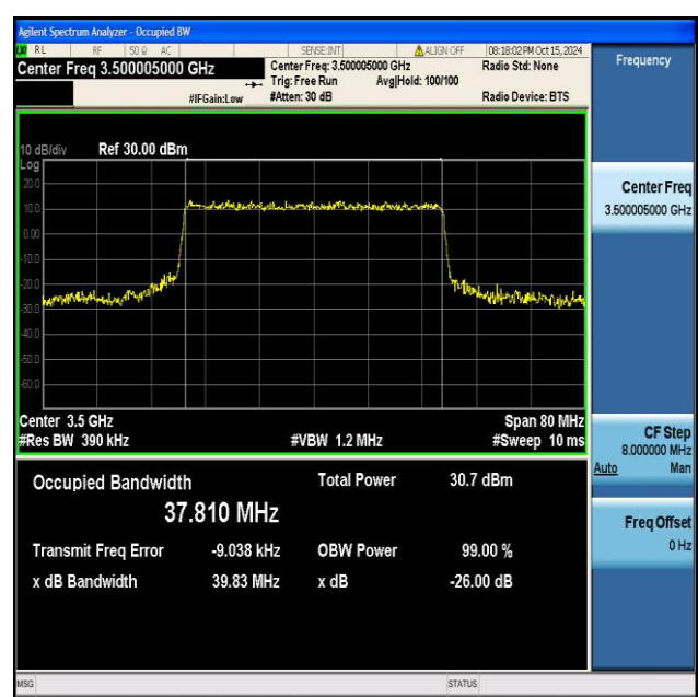
NTNV_N77-3450-3550_PC2_30_40_M_TID8_Ant1#1
