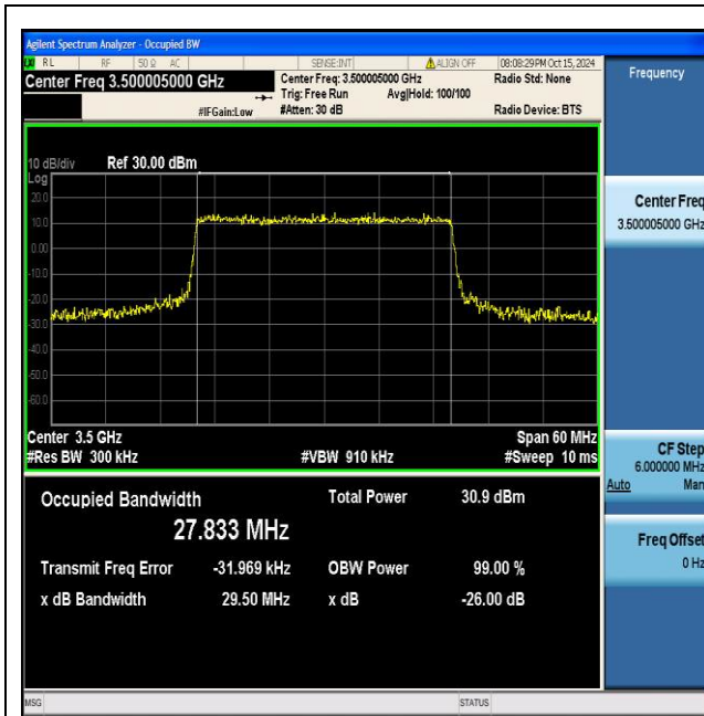
NTNV_N77-3450-3550_PC2_30_30_M_TID5_Ant1#1
