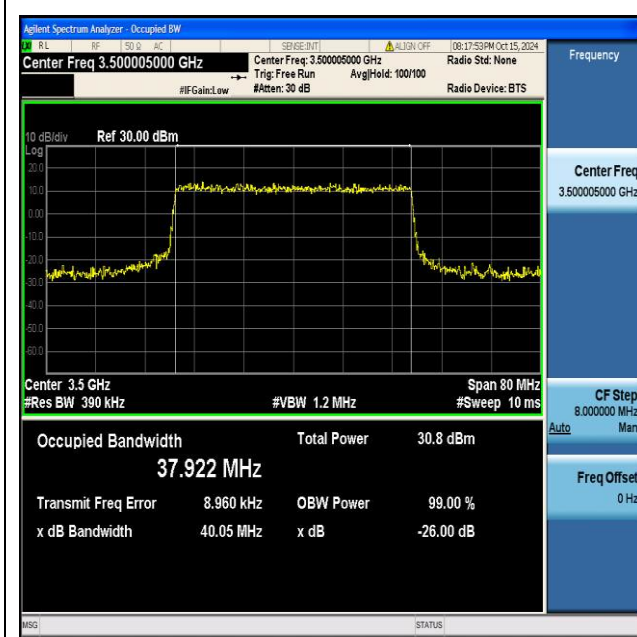
NTNV_N77-3450-3550_PC2_30_40_M_TID7_Ant1#1
