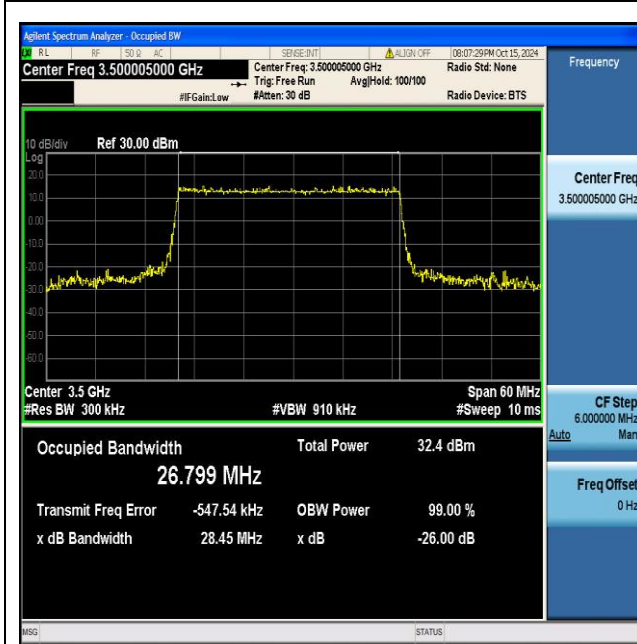
NTNV_N77-3450-3550_PC2_30_30_M_TID3_Ant1#1
