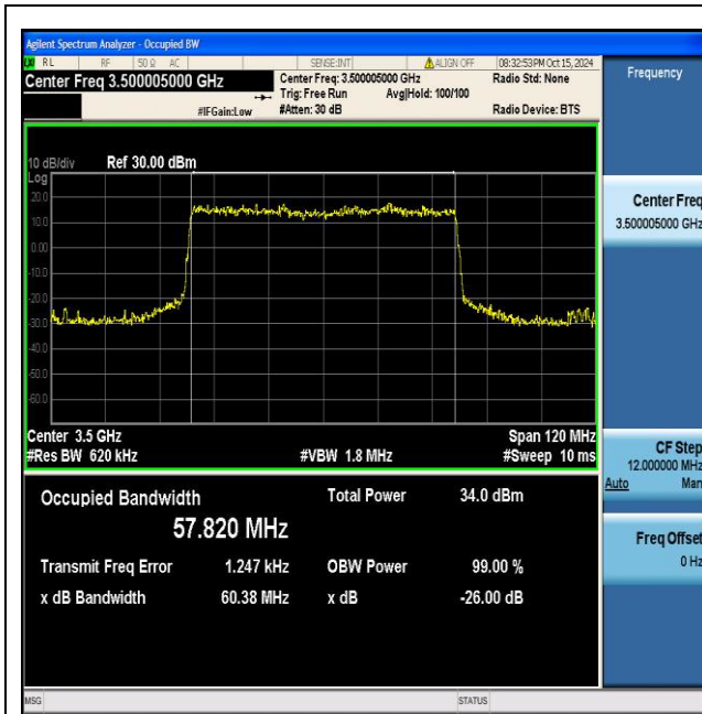
NTNV_N77-3450-3550_PC2_30_60_M_TID1_Ant1#1
