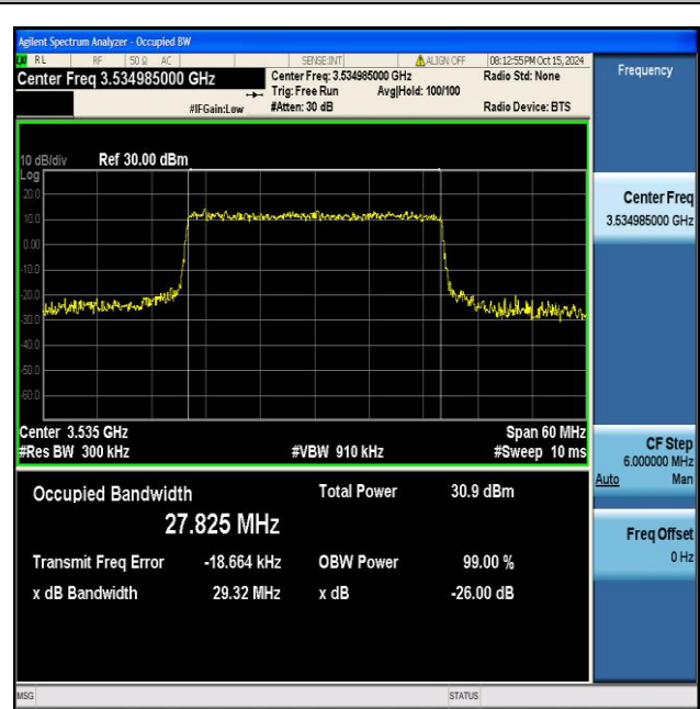
NTNV_N77-3450-3550_PC2_30_30_H_TID8_Ant1#1
