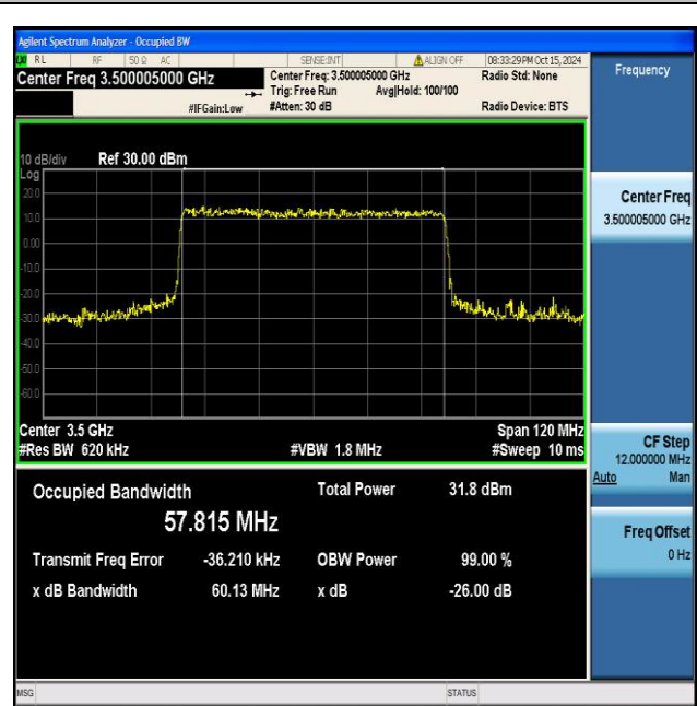
NTNV_N77-3450-3550_PC2_30_60_M_TID4_Ant1#1
