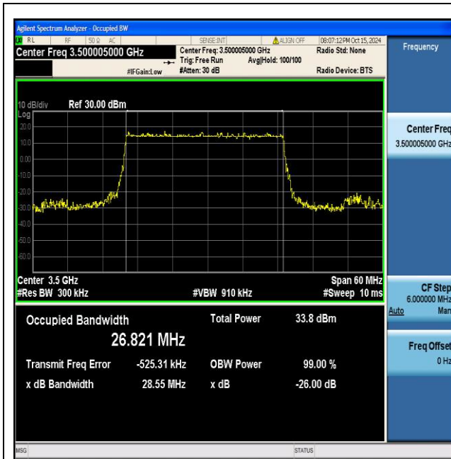
NTNV_N77-3450-3550_PC2_30_30_M_TID1_Ant1#1
