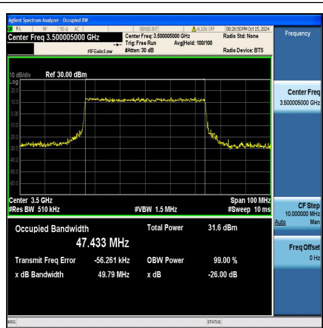
NTNV_N77-3450-3550_PC2_30_50_M_TID6_Ant1#1
