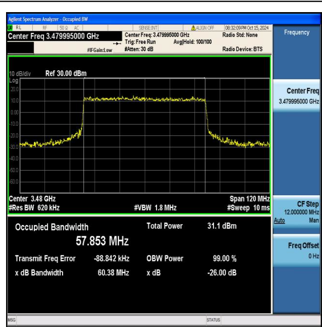
NTNV_N77-3450-3550_PC2_30_60_L_TID8_Ant1#1
