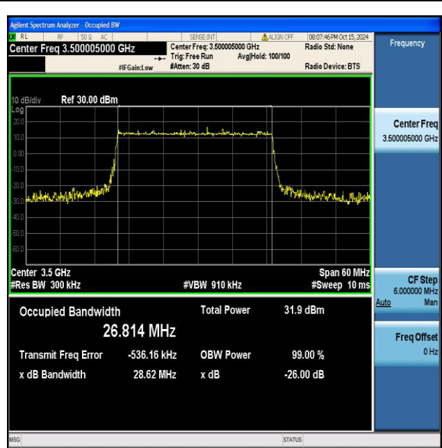
NTNV_N77-3450-3550_PC2_30_30_M_TID4_Ant1#1
