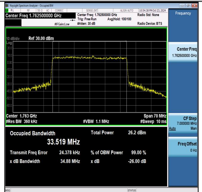
NTNV-n66-PC3-15-35-H-CP-256QAM-Outer_Full-Ant1-PASS
