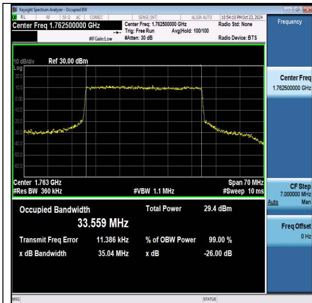
NTNV-n66-PC3-15-35-H-CP-QPSK-Outer_Full-Ant1-PASS
