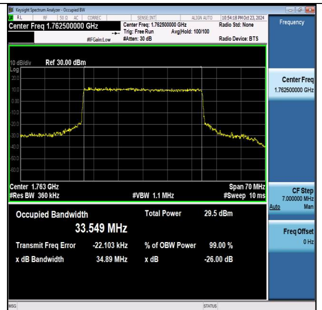
NTNV-n66-PC3-15-35-H-CP-16QAM-Outer_Full-Ant1-PASS
