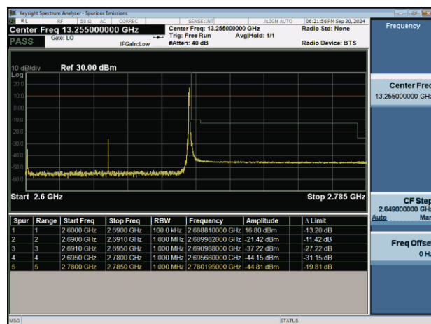
NTNV-n41-PC2-30-90-H-CP-QPSK-Edge_1RB_Right-PASS
