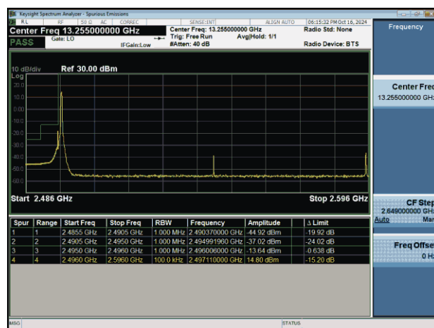
NTNV-n41-PC2-30-100-L-DFT-BPSK-Edge_1RB_Left-PASS
