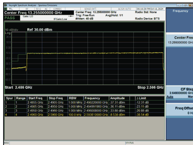
NTNV-n41-PC2-30-100-L-CP-QPSK-Outer_Full-PASS
