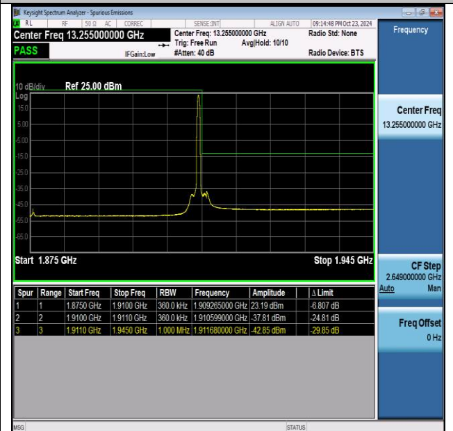
NTNV-n2-PC3-15-35-H-DFT-PI2BPSK-Edge_1RB_Right-PASS
