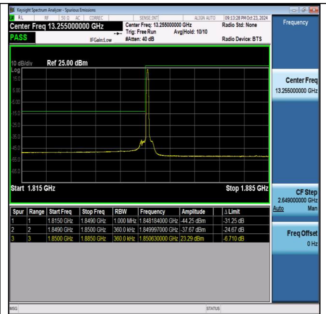
NTNV-n2-PC3-15-35-L-DFT-PI2BPSK-Edge_1RB_Left-PASS
