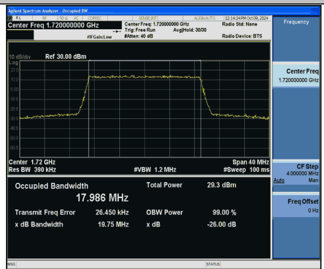
Band66-20MHz-256QAM-132072-100RB#0-PASS
