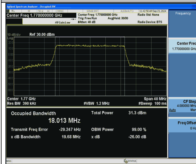
Band66-20MHz-64QAM-132572-100RB#0-PASS
