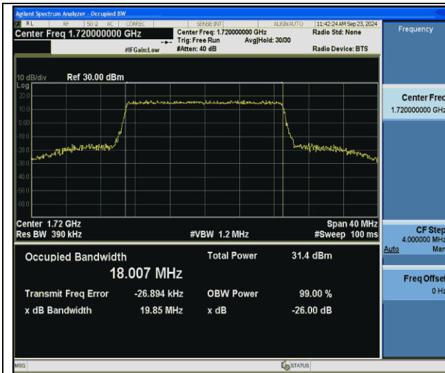
Band66-20MHz-64QAM-132072-100RB#0-PASS
