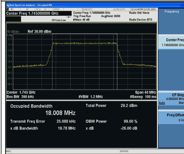
Band66-20MHz-256QAM-132322-100RB#0-PASS
