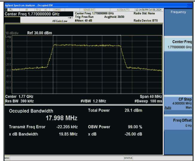
Band66-20MHz-256QAM-132572-100RB#0-PASS
