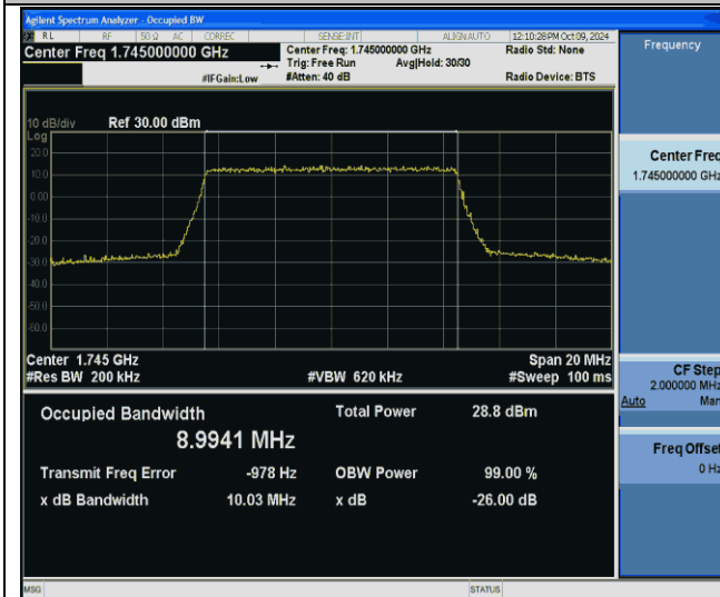
Band66-10MHz-256QAM-132322-50RB#0-PASS
