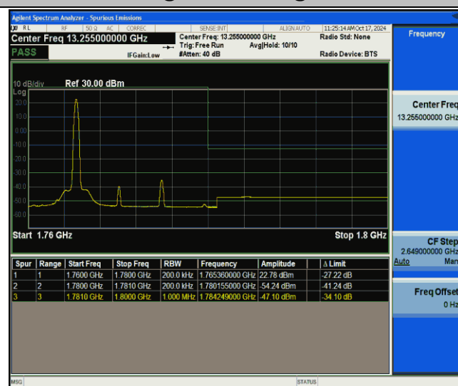
66-66-5MHz-15MHz-QPSK@QPSK-QPSK@QPSK-132504-132597-1RB#24@25RB#0-0RB#0@75RB#0-PASS
