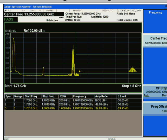
66-66-5MHz-15MHz-QPSK@QPSK-QPSK@QPSK-132504-132597-1RB#0@25RB#0-1RB#74@75RB#0-PASS
