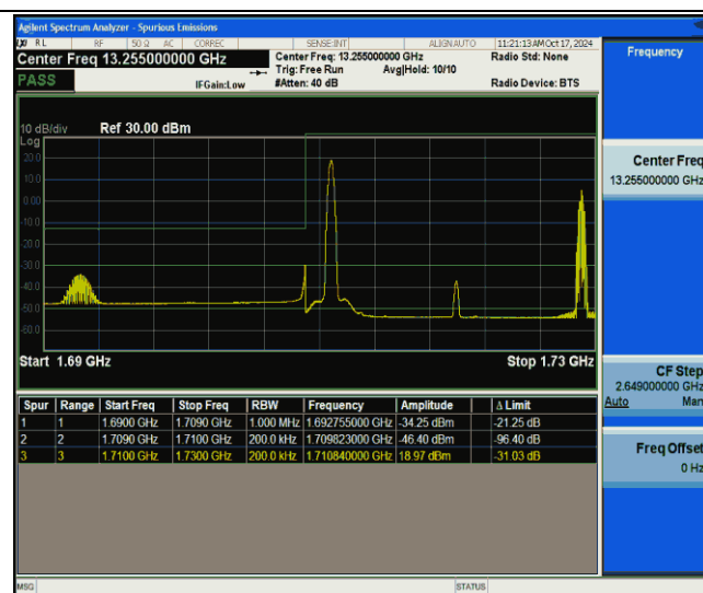
66-66-5MHz-15MHz-QPSK@QPSK-QPSK@QPSK-132002-132095-1RB#0@25RB#0-1RB#74@75RB#0-PASS
