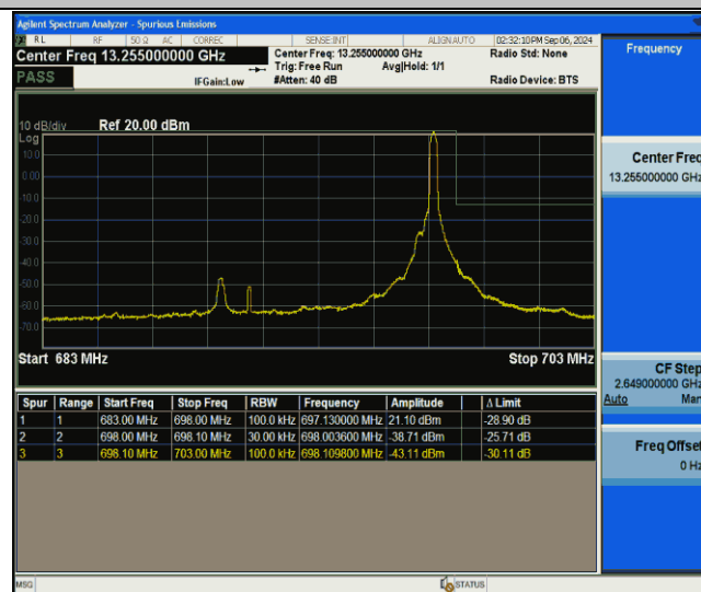
Band71-15MHz-QPSK-133397-1RB#74-PASS
