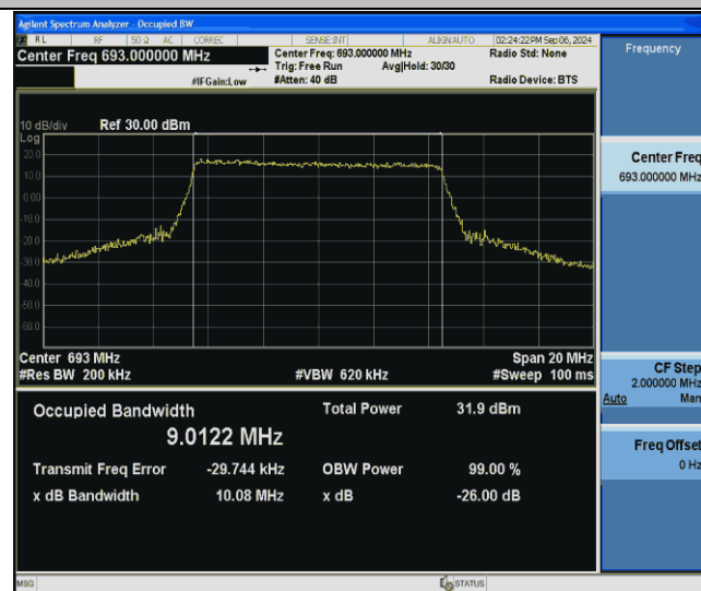
Band71-10MHz-16QAM-133422-50RB#0-PASS
