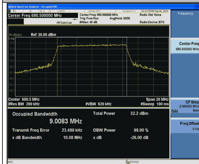
Band71-10MHz-16QAM-133297-50RB#0-PASS
