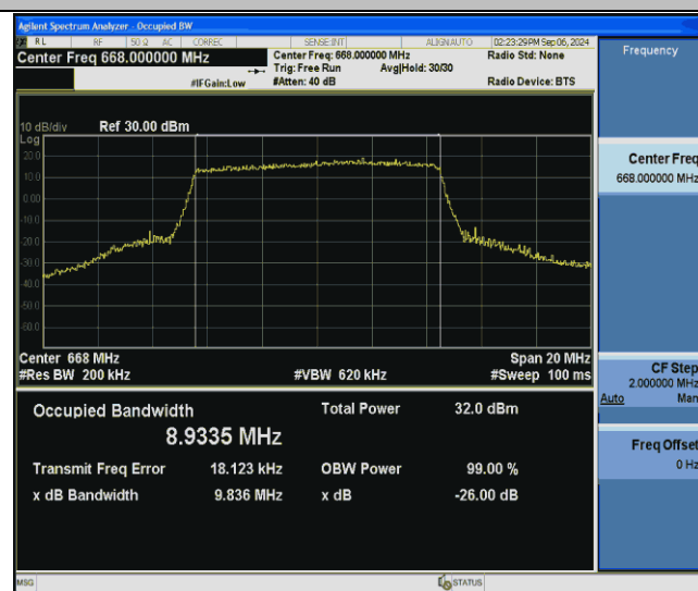
Band71-10MHz-16QAM-133172-50RB#0-PASS
