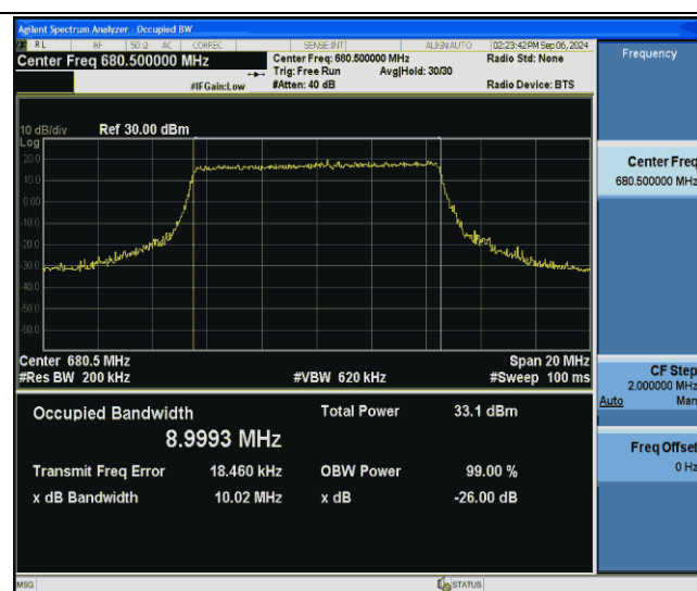
Band71-10MHz-QPSK-133297-50RB#0-PASS
