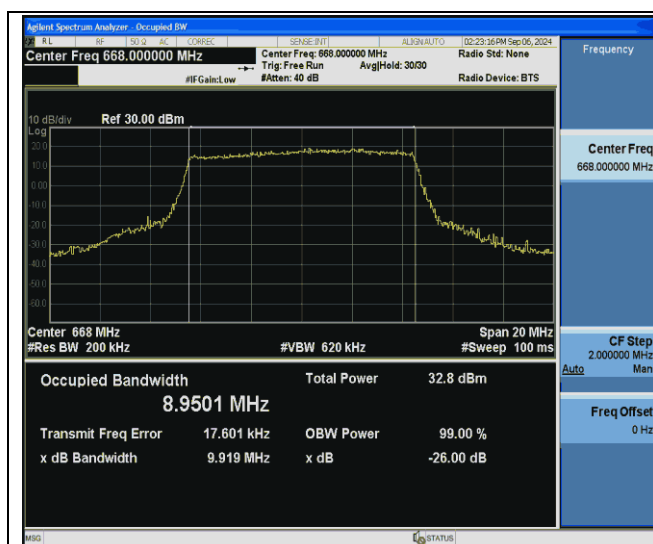
Band71-10MHz-QPSK-133172-50RB#0-PASS
