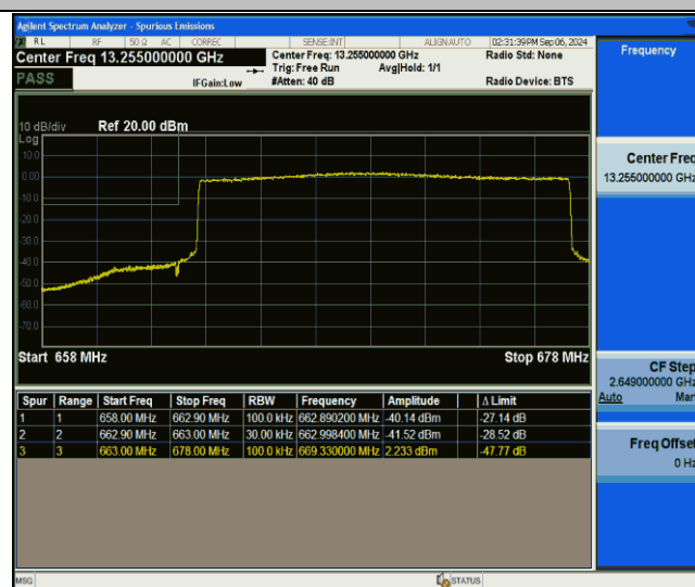
Band71-15MHz-QPSK-133197-75RB#0-PASS
