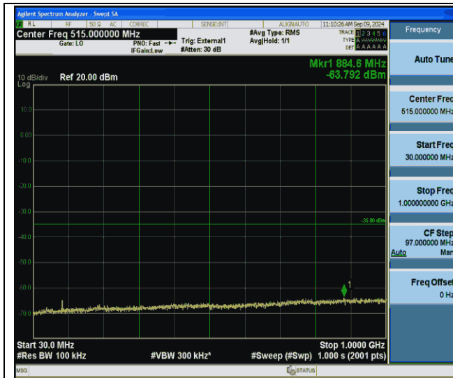
Band41-20MHz-QPSK-41490-1RB#0-30~1000-PASS
