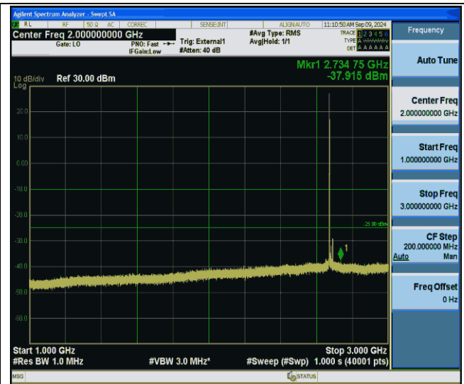
Band41-20MHz-QPSK-41490-1RB#0-1000~3000-PASS
