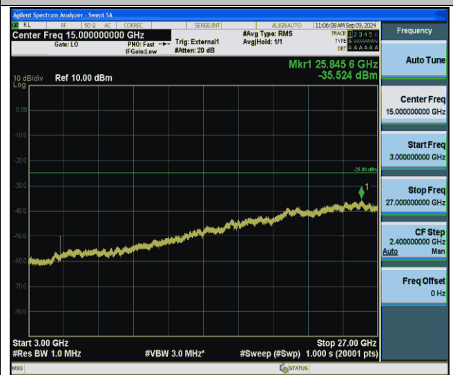
Band41-20MHz-QPSK-40620-1RB#0-3000~27000-PASS
