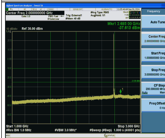
Band41-20MHz-QPSK-40620-1RB#0-1000~3000-PASS
