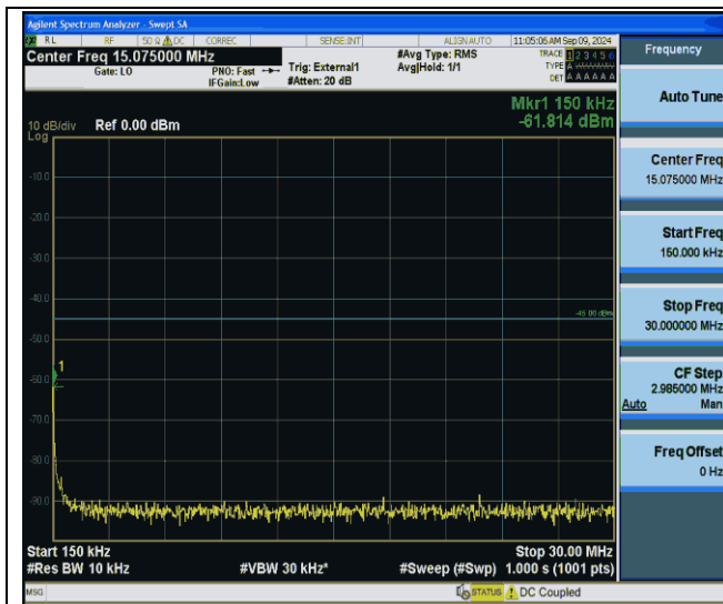
Band41-20MHz-QPSK-40620-1RB#0-0.15~30-PASS
