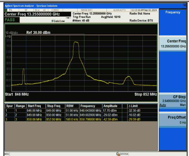
Band26(824-849)-5MHz-QPSK-27015-1RB#24-PASS
