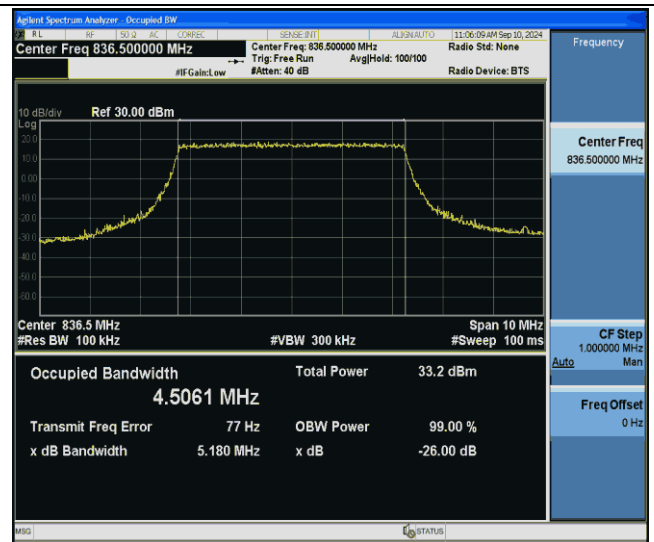
Band26(824-849)-5MHz-QPSK-26915-25RB#0-PASS
