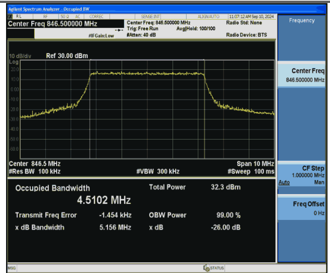
Band26(824-849)-5MHz-16QAM-27015-25RB#0-PASS
