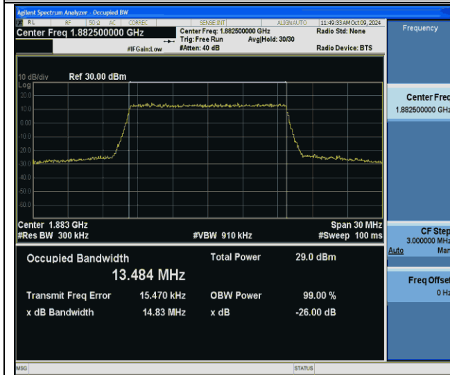
Band25-15MHz-256QAM-26365-75RB#0-PASS
