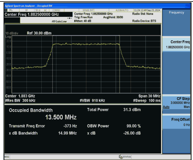
Band25-15MHz-64QAM-26365-75RB#0-PASS
