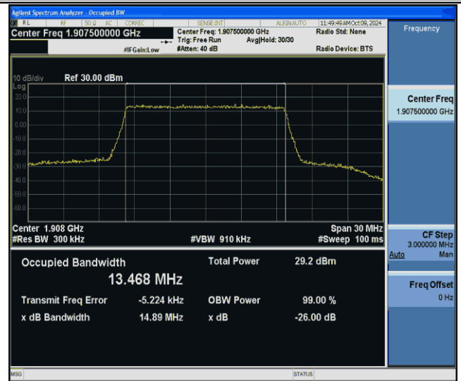
Band25-15MHz-256QAM-26615-75RB#0-PASS
